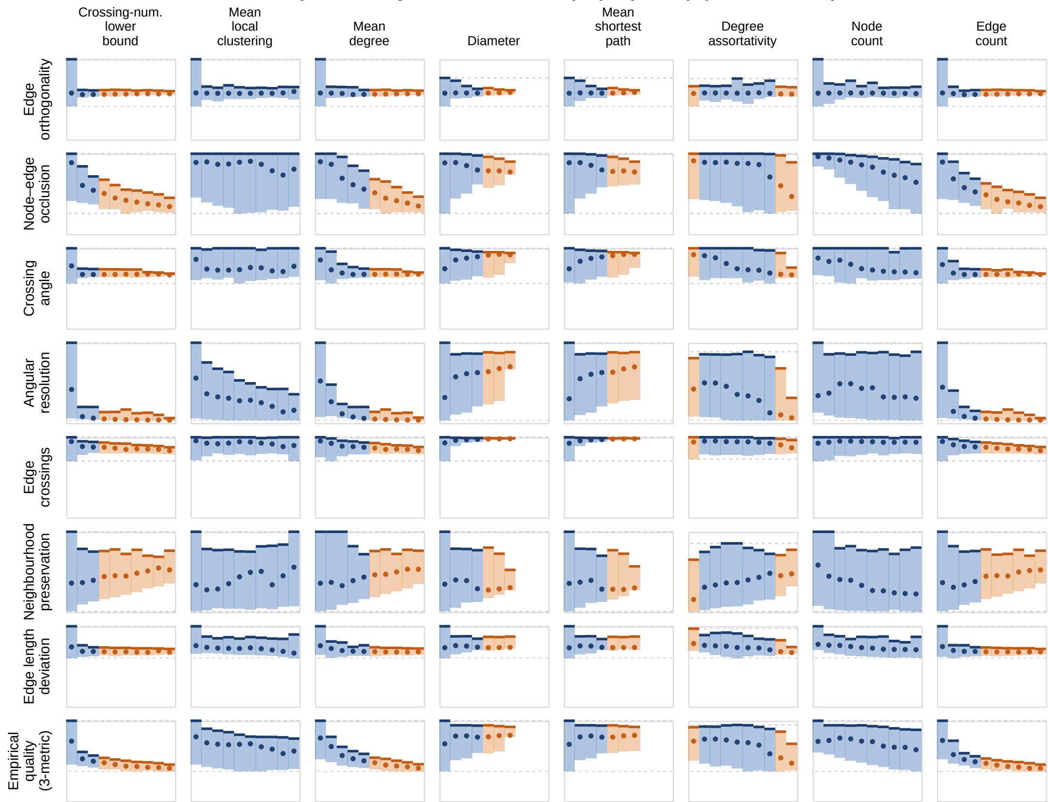
Readability metric ranges across structural-property bins (equal-width, n=10)
