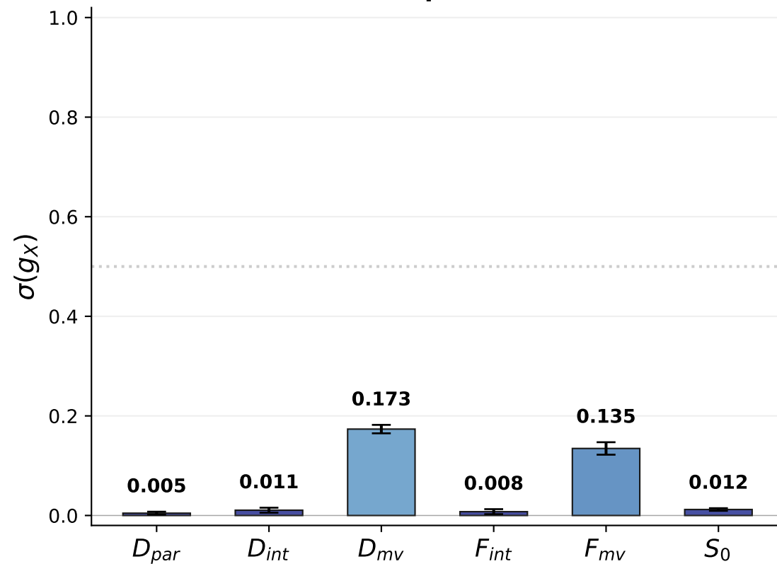
PACE: Learned Spatial Gate Values
