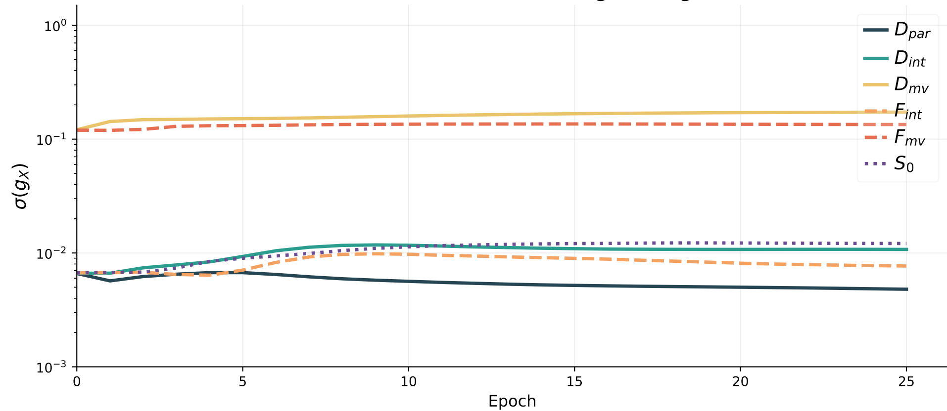
CNN Fusion: Gate Evolution During Training
