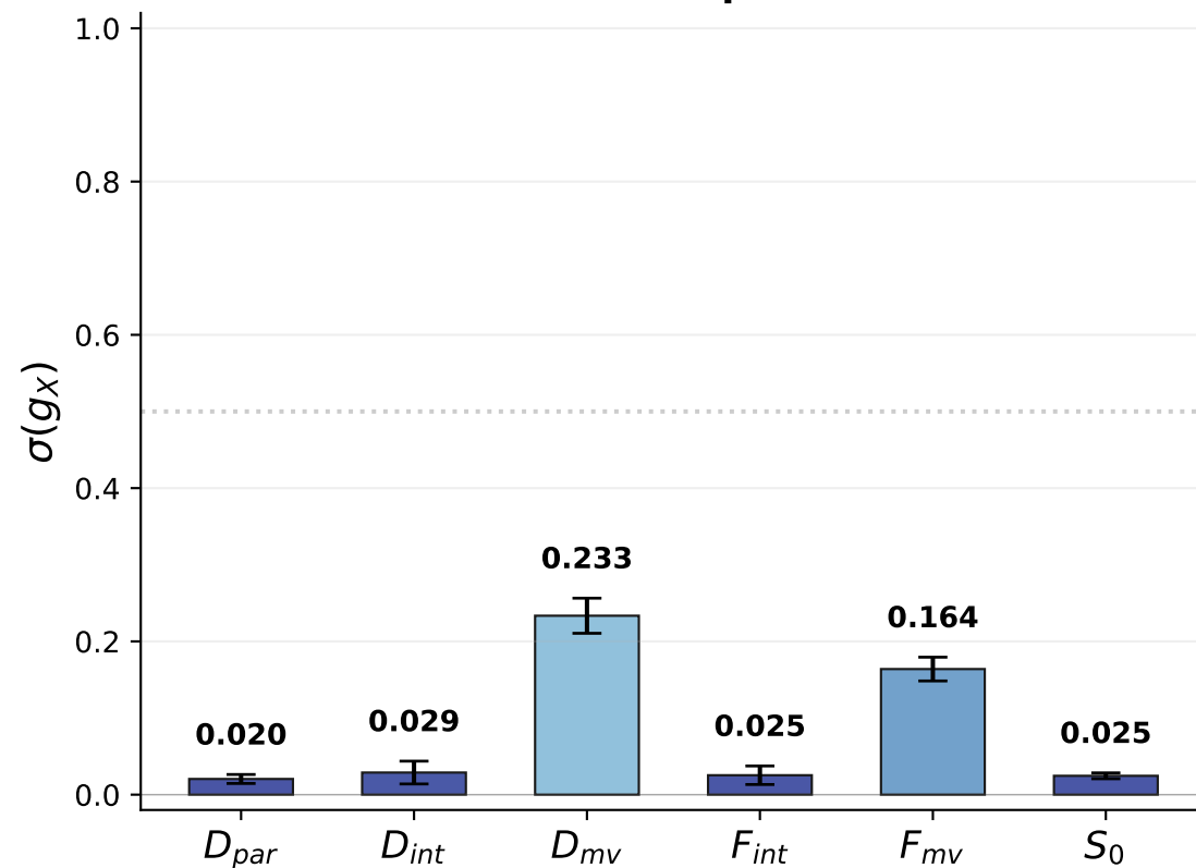
CNN Fusion: Learned Spatial Gate Values
