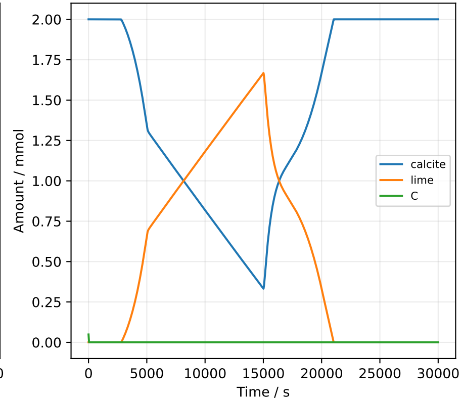
Cell plus both reservoirs
