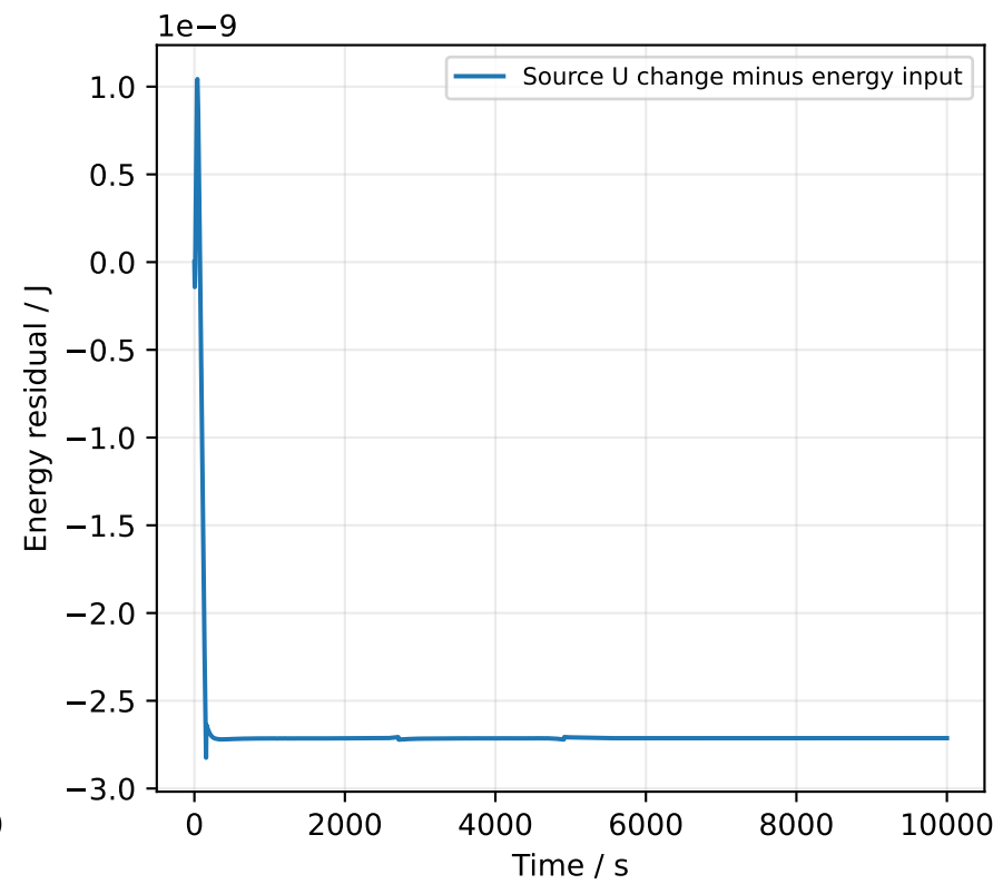
Numerical balance at saved observations
