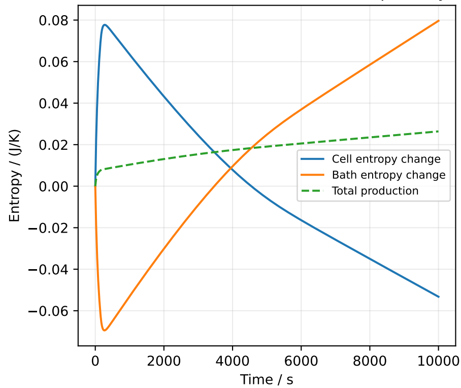
Cell and external bath accounted separately
