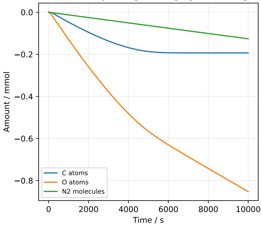
Net inventory change through gas exchange
