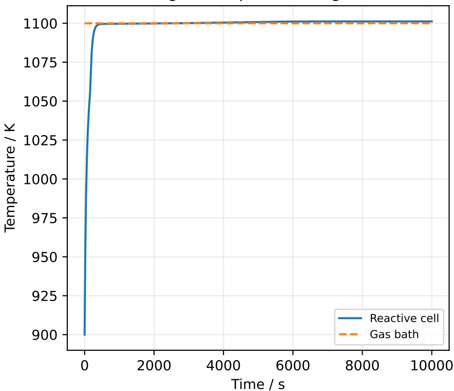
Heating with a prescribed gas bath
