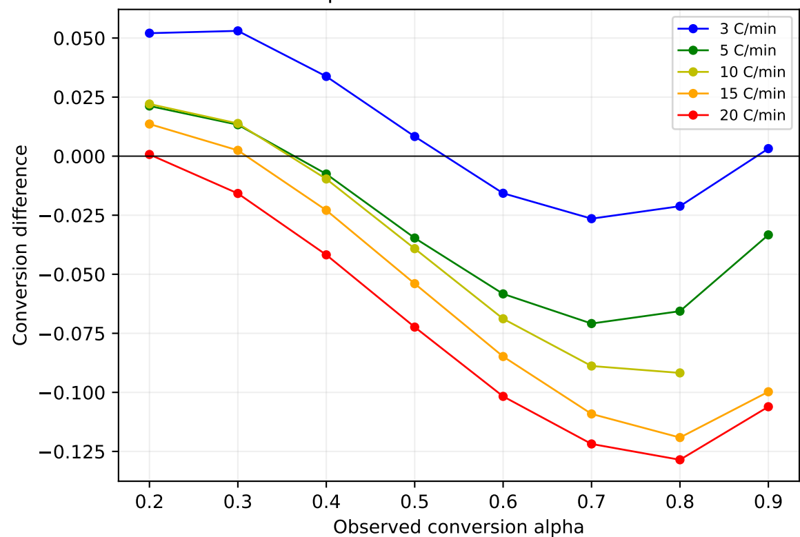
SRB: prediction minus observation
