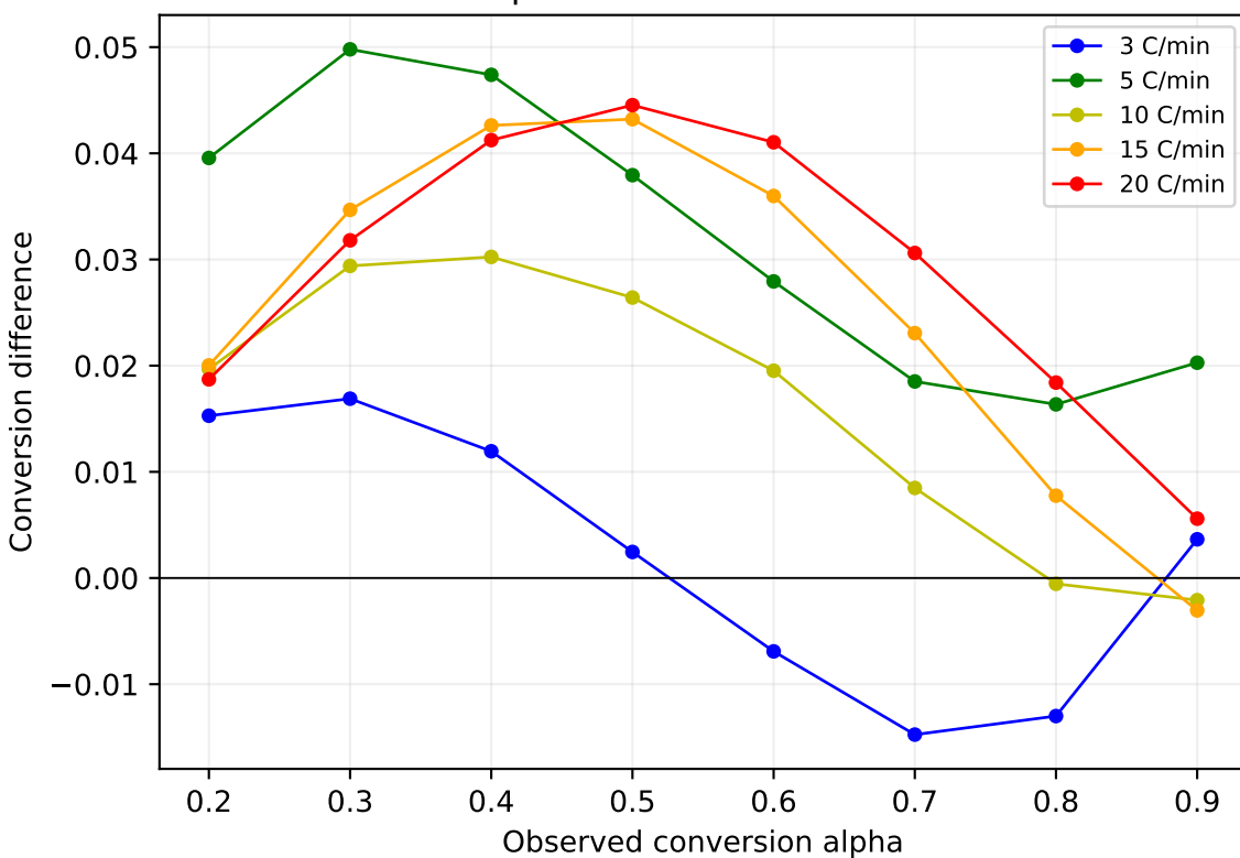
KGa-1: prediction minus observation
