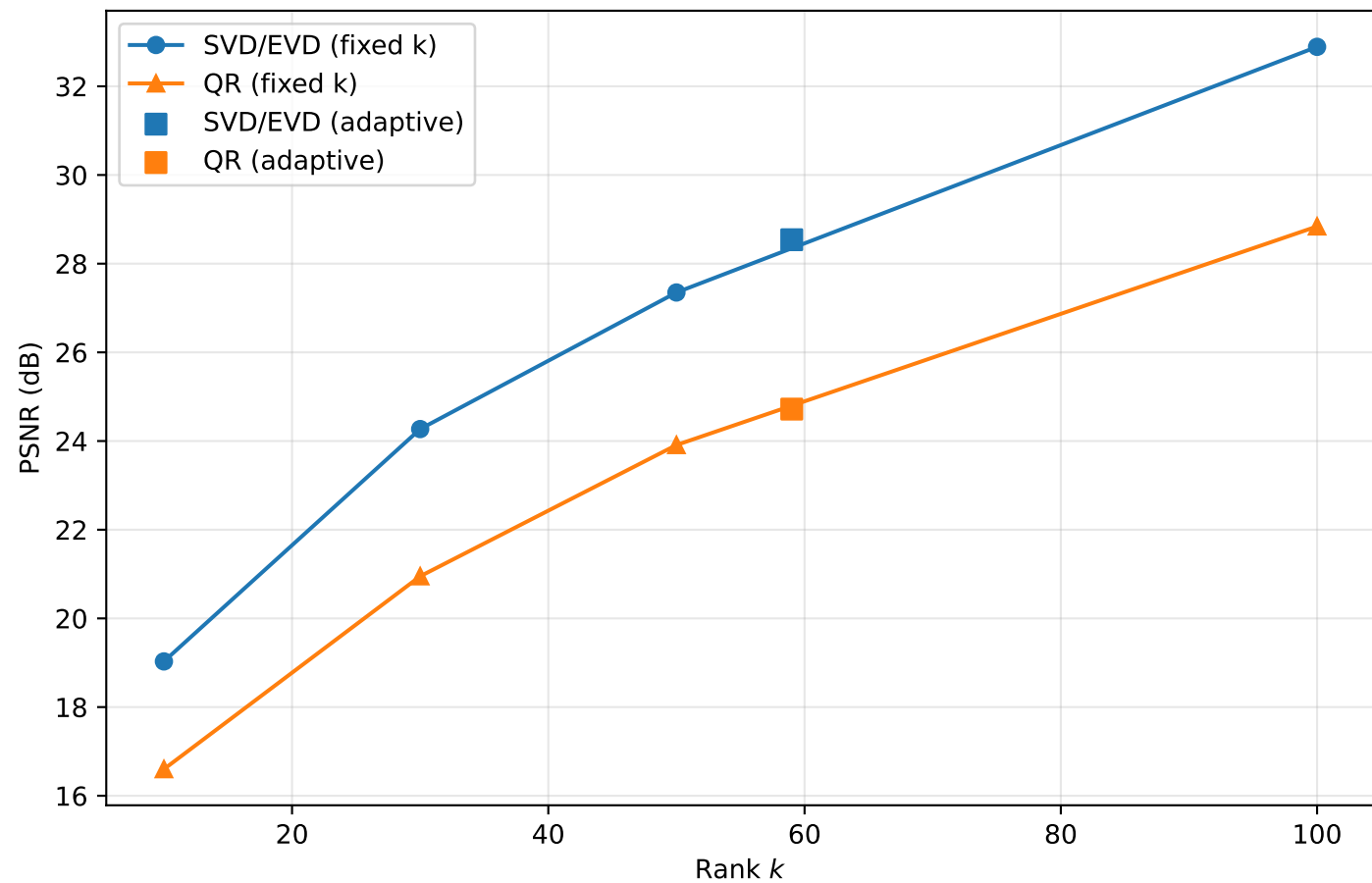
PSNR vs. Rank k for SVD/EVD and QR (Fixed and Adaptive)
