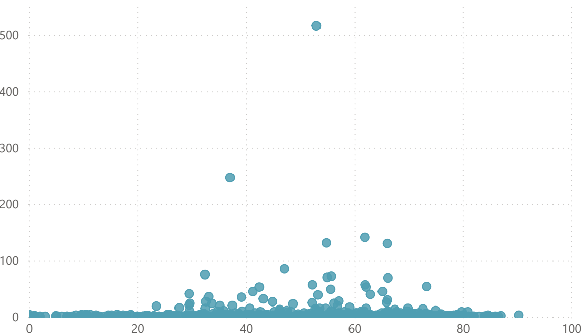
Average Popularity and Count of track_duration_min by artist_genres
