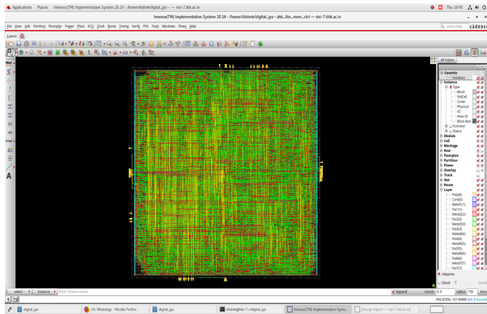
Figure 7: 2D Physical Layout view of the placed and routed design in Cadence Innovus.
