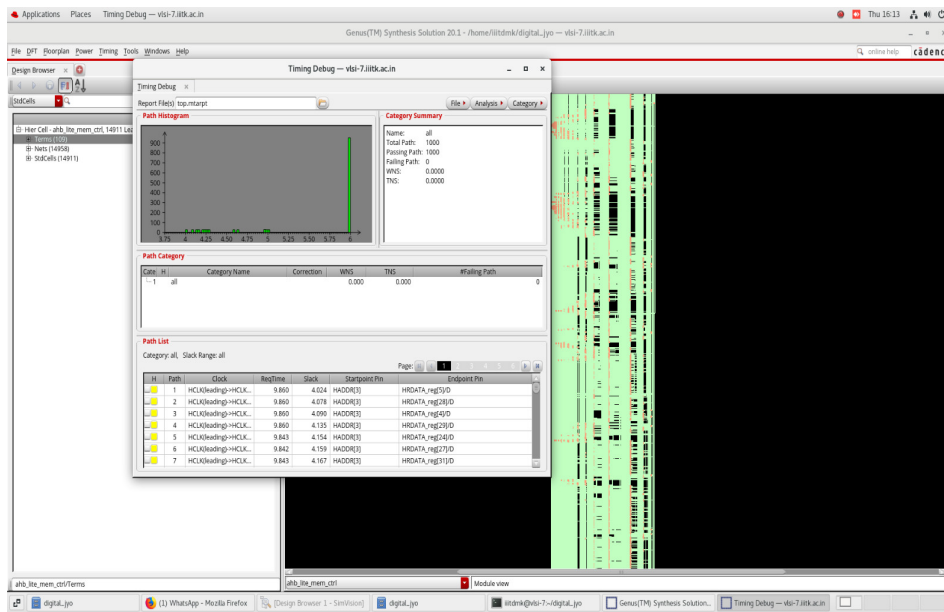
Figure 5: Timing Report generated after synthesis showing slack and critical path delay.
