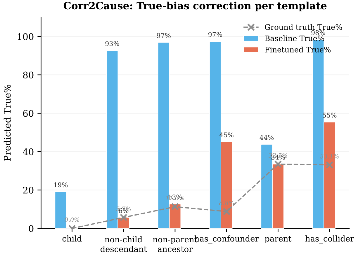
Figure 2: Corr2Cause True-bias correction per template. The baseline predicts True at rates far exceeding ground truth (e.g., 98.4% vs 33.1% on has_collider). The finetuned model corrects this bias, tracking ground truth closely.
