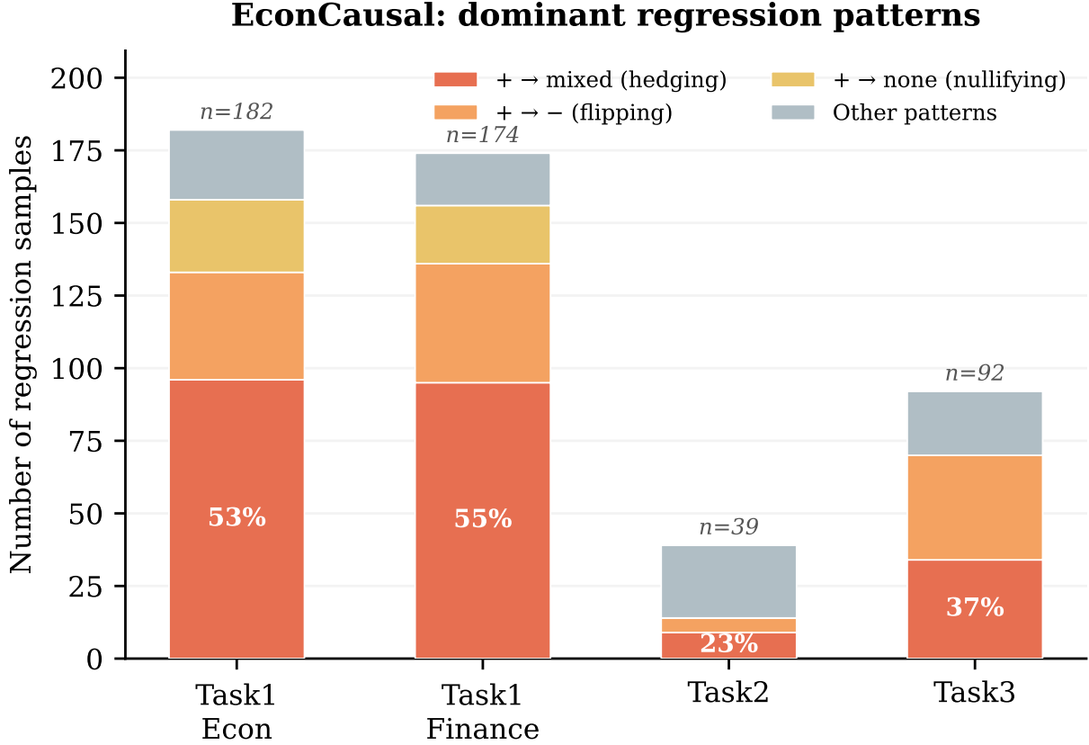
Figure 3: EconCausal dominant regression patterns. Positive-to-mixed hedging ( + \rightarrow mixed) accounts for 53% of Task1 Econ regressions and 55% of Task1 Finance regressions, making it the dominant failure mode.
