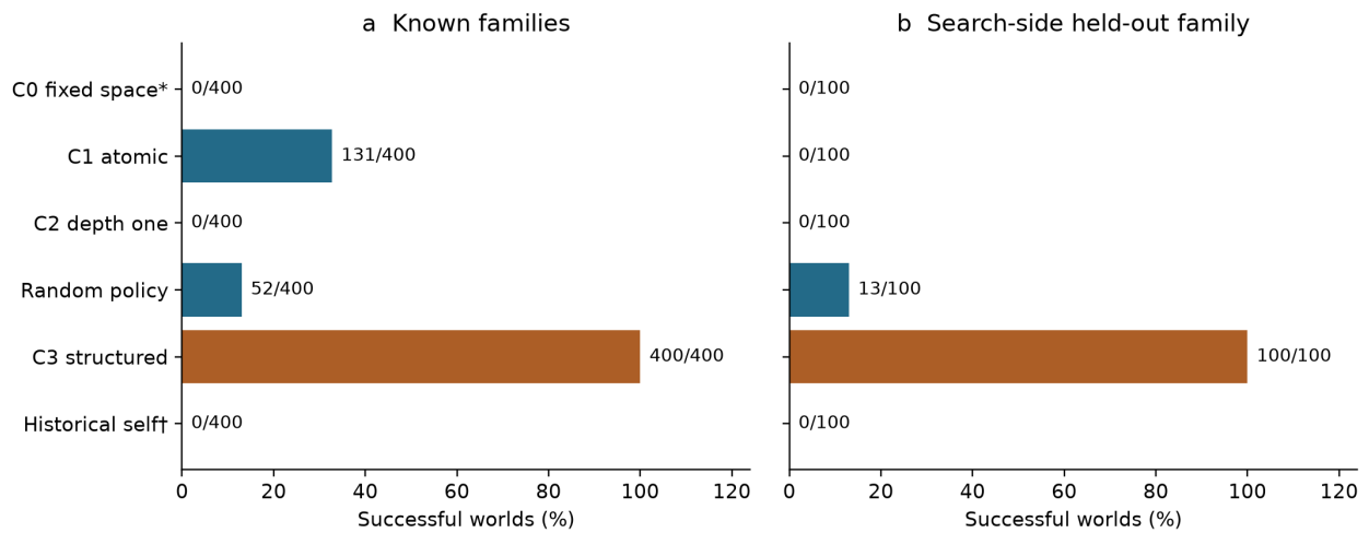
Figure 3. Generic search under a fixed realization language. Known-family and search-side held-out world counts have different denominators. C0 (*) is a structural control; historical self-composition (†) is interface-confounded. The C3/random contrast includes traversal and selection, not proposal source alone. The held-out algebraic basis was already supplied.
