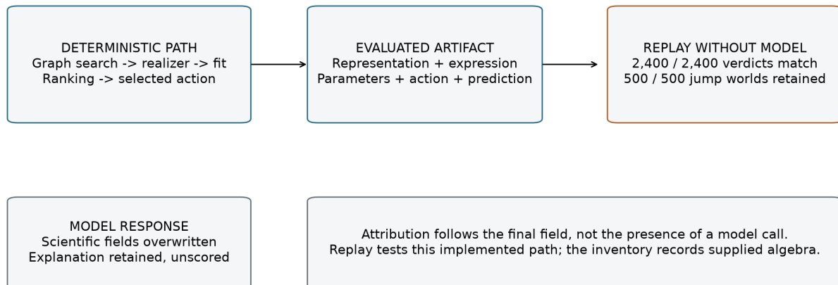
Figure 4. C3 evaluated-field provenance and post-hoc replay. Scientific model fields are overwritten before scoring; the retained explanation does not enter the gates. Removing model outputs preserves all candidate verdicts and all jump-world successes, alongside zero control successes. Schematic prepared with ChatGPT/Codex assistance and rendered programmatically.
