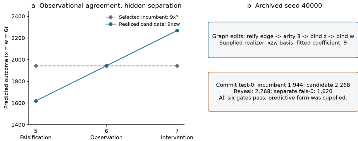
Figure 7. Reconstructing the worked prospective example in Section 5.1. Archived held-out seed 40000 supplies the observations, committed test-0 and separate fals-0 outcome. The plotted slice fixes x=w=6 . The complete falsification split also includes a second case, used in the all-gate verdict. The graph leaves the structural language; its product basis is supplied by the realizer. Figure prepared with AI-assisted code from the archived candidate and deterministic world reconstruction.
