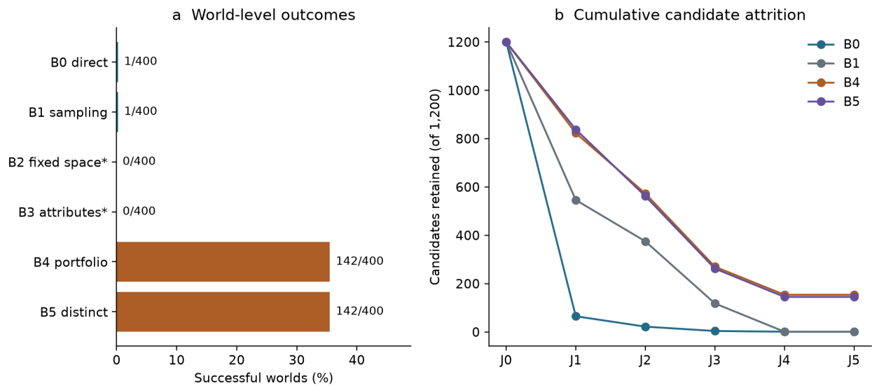
Figure 2. Representation-level proposals under the prospective assay. (a) World success counts, n=400 per condition. Asterisks mark fixed-language structural controls whose reachable graphs cannot pass J1. (b) Cumulative gate retention among 1,200 candidates per condition; candidates are not independent replicates. Rates and bootstrap intervals are available in the source data. Figures 2, 3, 5 and 6 are reproducible plots of frozen artifacts, prepared with AI-assisted plotting code.
