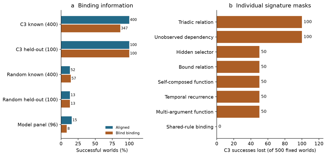
Figure 6. Dependence on binding information and supplied signatures. (a) Aligned versus role/action-blind binding; annotations are successful-world counts and denominators appear in labels. (b) C3 world successes lost under each individual signature mask, combining 400 known and 100 held-out worlds. The triadic loss is confined to the holdout. All interventions fix archived candidate slots; no adaptive re-search occurs. Incumbent substitution is retained only as a structural negative control in the supplement.
