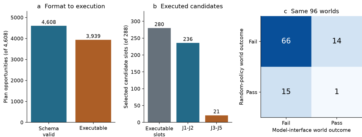
Figure 5. Grammar-interface sensitivity. Plan opportunities (a), selected candidate slots (b) and paired worlds (c) are distinct units. Of 288 slots, 280 contain an executable selected plan; 236 pass J1-J2 and 21 pass J3-J5. The paired panel contains 96 worlds, with model and random successes in 15 and 16 respectively. Format repair exposes evaluated topology without an aggregate model advantage.
