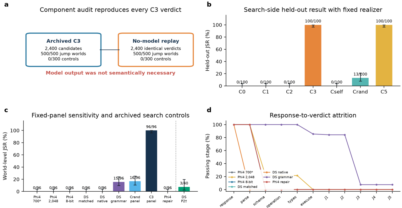
Figure 4 | Component attribution, held-out transfer and targeted sensitivity. Panel a compares archived C3 verdicts with inference-free replay; all 2,400 candidate verdicts matched. Panel b reports held-out JSR with Wilson 95% intervals for n=100 worlds. Panel c reports the fixed n=96 sensitivity panel and archived C_rand/C3 controls; the supplied-representation control (dagger) uses a distinct balanced n=40 subset. Panel d reports response-to-verdict attrition; denominators change from responses or plan opportunities to executable selected candidates at J1. Connecting lines show stage order, not a common denominator. No candidate-level significance tests were performed.
