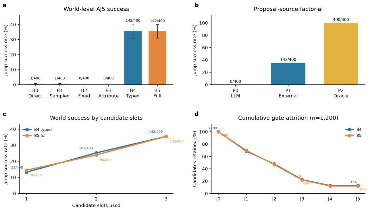
Figure 2 | Typed proposals and their gate attrition. Panels a and b report world-level jump success rate (JSR) for n=400 worlds per condition; intervals are registered family-stratified bootstrap 95% intervals. Panel c reports cumulative successful-world counts and rates as one, two and three slots are admitted. Panel d reports cumulative candidate retention from J0 to J5 for 1,200 candidates per condition; candidates are not independent replicates. All AJ5 conditions recorded 0/200 control-world false jumps.
