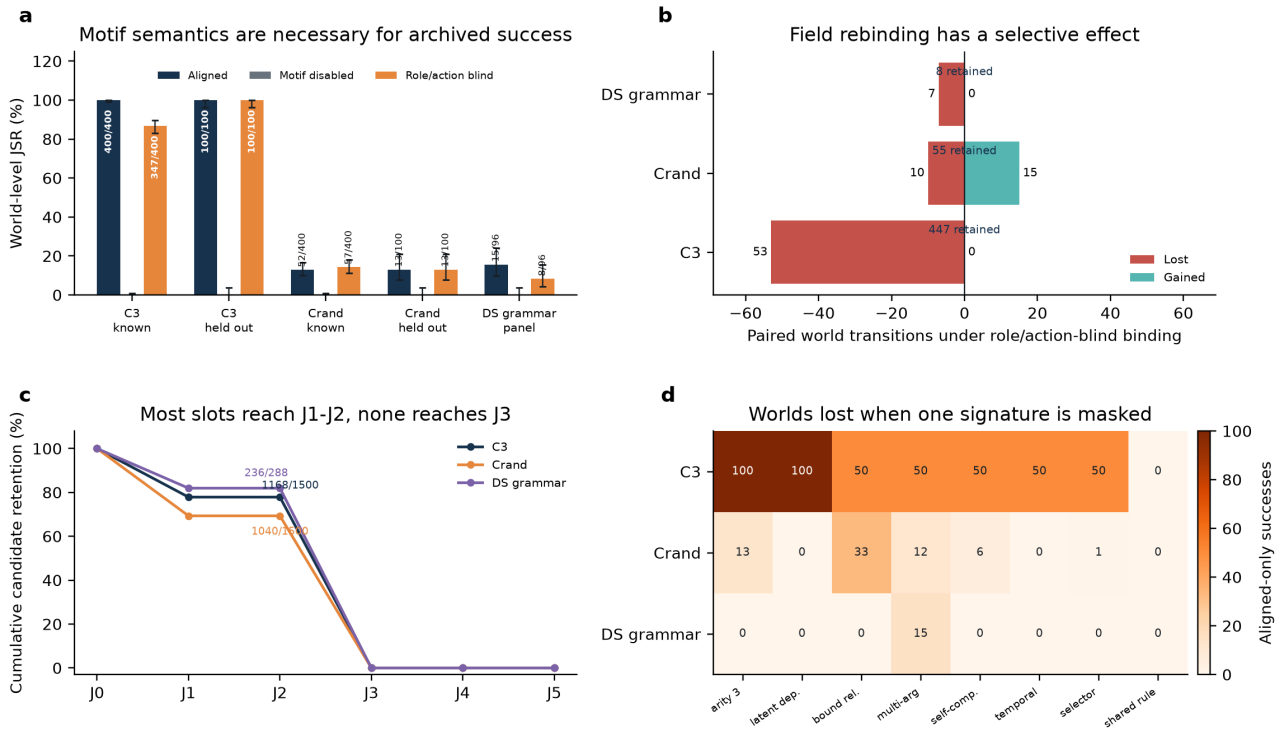
Figure 5 | Counterfactual dependence on motif semantics. Panel a reports exact world-level jump success rates with Wilson 95% intervals under aligned, motif-disabled and role/action-blind realization. Panel b gives paired transitions from aligned to role/action-blind binding; counts pool 400 known-family and 100 held-out worlds for C3 and C_rand, while DeepSeek uses the fixed n=96 panel. Panel c reports cumulative candidate-slot attrition when motif realization is disabled; candidate slots are not independent replicates. Panel d reports aligned successes lost when one detected signature is replaced by incumbent fallback. Candidate representations and slots were fixed from the aligned archive; the post-confirmatory audit made zero model calls and did not rerun search under counterfactual realizers.
