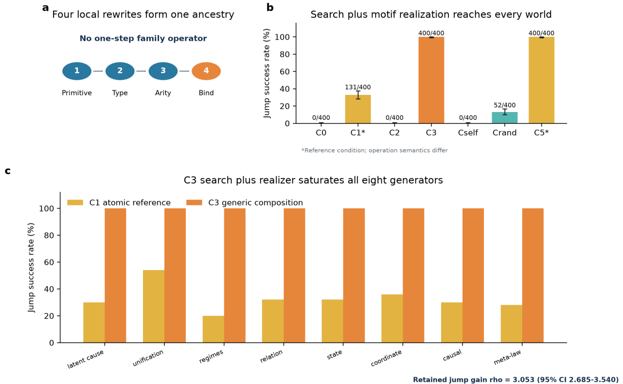
Figure 3 | Generic search with fixed motif realization. Panel a is schematic. Panel b reports known-family JSR with Wilson 95% intervals for n=400 worlds per condition. C1 and C5 are reference conditions with different operation semantics. Panel c reports descriptive rates for 50 worlds per family. C3 combines generic edit search with a fixed motif-to-basis realizer; saturation is within-generator reliability, not independent family replication.
