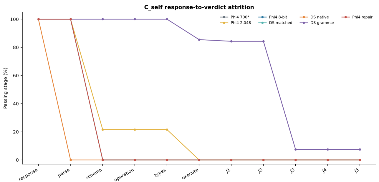
Extended Data Figure 8b | Response-to-verdict attrition, including the grammar-constrained interface cascade. Denominators and units change at the executable boundary and are reported in the accompanying source-data tables.
