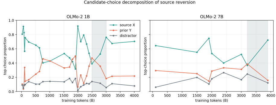
Figure S2. Candidate-choice decomposition across the complete OLMo-2 trajectories. Lines show item-cluster means for the explicit source, parametric prior, and distractors; shaded regions mark the selected late transitions.
