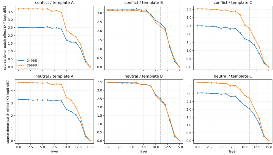
Figure S3. Layer-wise source-donor patch effect for conflict and neutral items at the OLMo-2 1B 2496B-to-2999B transition. The dashed line marks the first-75%-depth summary boundary.
