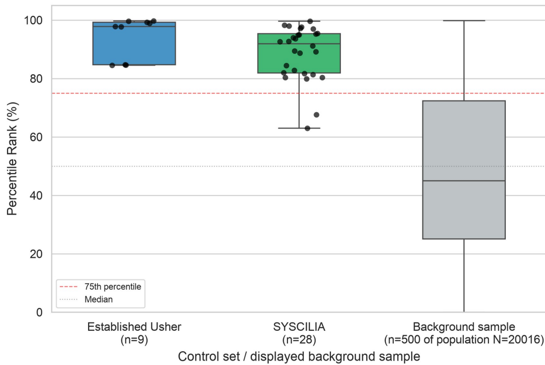
Figure 5. Internal control recovery. Percentile-rank distributions for the nine established Usher genes, the 28 SYSCILIA ciliary genes, and a sample of 500 non-control scored background genes drawn without replacement with numpy.random.default_rng(42) after ordering eligible labels by retained Ensembl ID, shown as box plots with the controls also plotted as individual points. The dashed line marks the 75th percentile and the dotted line the median. The control set is curated and is not an independent validation cohort.
