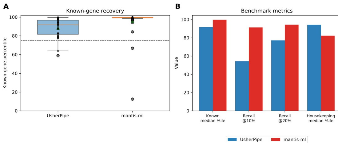
Figure 9. Exploratory benchmark against mantis-ml. (A) Percentile-rank distributions of the 35 curated controls shared by both tools' gene universes (shared universe: 16,821 labels). Black points show individual controls; boxes show interquartile ranges and median lines, whiskers extend to 1.5 times the interquartile range, open circles mark boxplot outliers and green triangles indicate means. The dashed line marks the 75th
