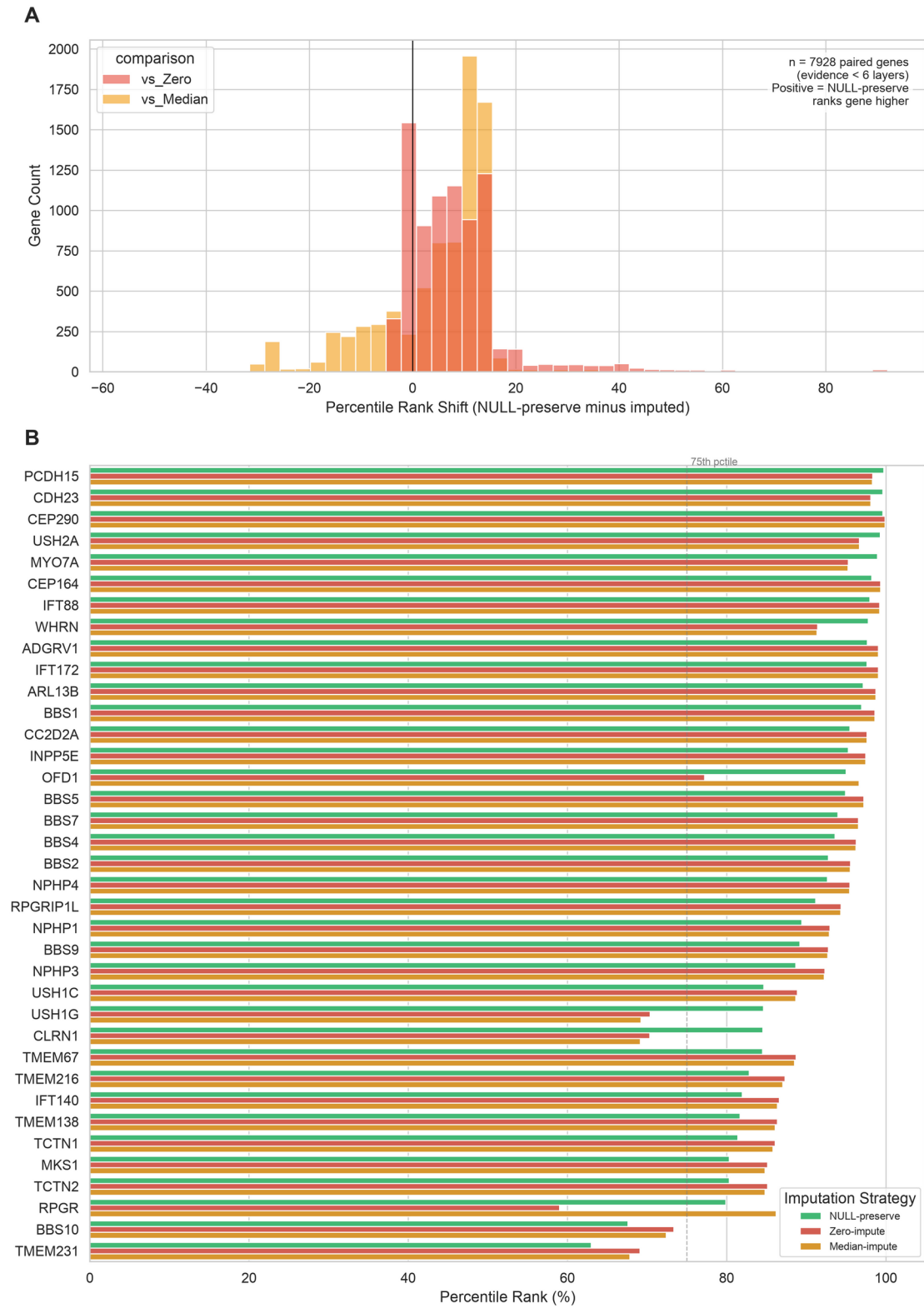
Figure 6. Effect of missing-data handling on rankings. (A) Distribution of percentile-rank shifts for labels with incomplete evidence under NULL-preservation relative to zero imputation and to median imputation; positive values indicate that NULL-preservation ranks the label higher. (B) Percentile rank of selected controls
