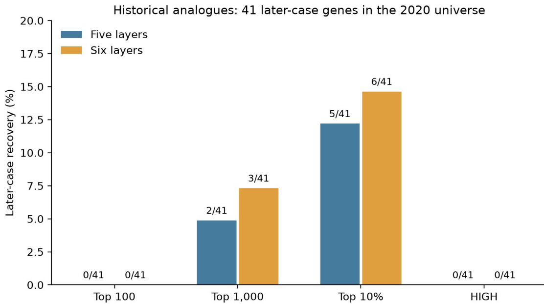
Figure 8. Retrospective recovery of later target associations. Five-layer archived and six-layer literature-augmented historical analogues evaluated the 41 principal cases in the 2020 protein-coding universe. Bars show deterministic top 100, top 1,000, top 10% and HIGH recovery; the numerators and denominator are labeled. Four additional noncoding cases remain failures in the 45-case end-to-end analysis (Table 4). Neither version recovers a principal case at top 100 or HIGH. These are retrospective source-analogue results, with post-cutoff method development and catalog-based ascertainment limitations.
