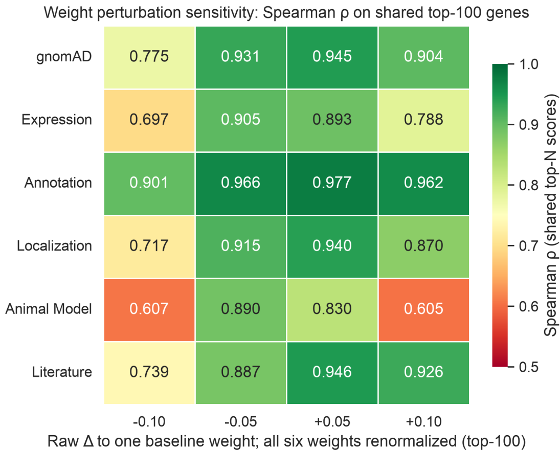
Figure 7. Sensitivity of rankings to weight perturbation. Spearman rank correlation and top-100 overlap metrics under 24 absolute weight-point perturbations (six layers, each changed by \pm 0.05 and \pm 0.10 ). Each raw delta was applied to one weight and then all six weights were renormalized, so the final change is not literally the raw delta and the other weights also change. Sixteen perturbations met \rho \geq 0.85 ; mean \rho was 0.8548 and the range was 0.6051–0.9770. On conditional top-100 correlation, animal-model perturbations were the most sensitive and annotation perturbations the least sensitive; this ordering does not describe whole-universe correlation or shortlist overlap; the top-100 Spearman statistic is conditional on overlapping genes.
