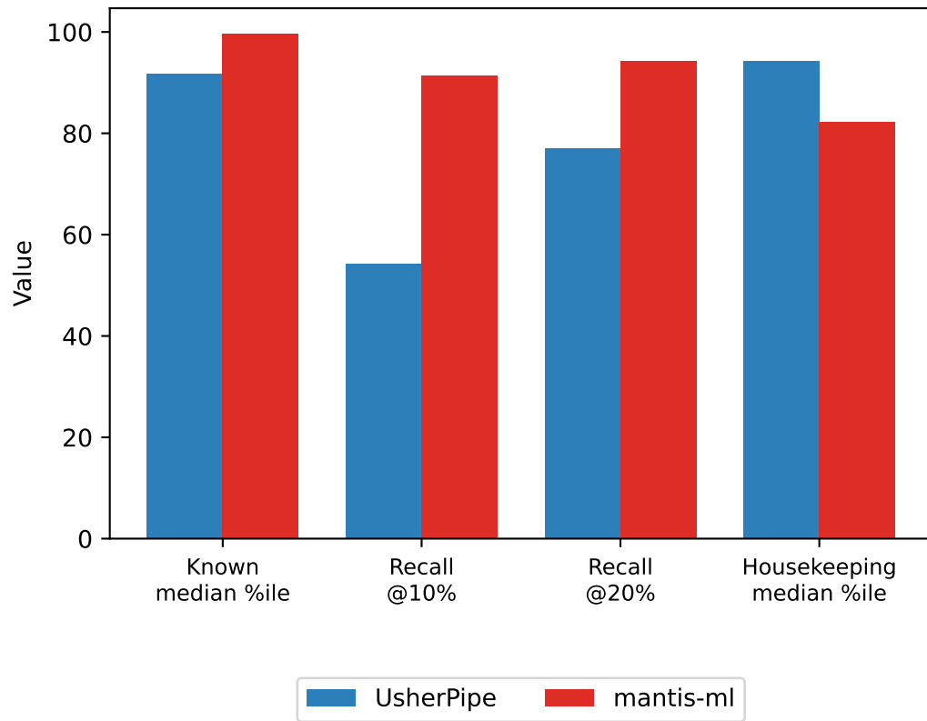
Benchmark metrics
