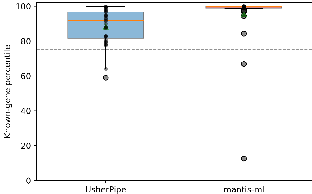
Known-gene recovery
