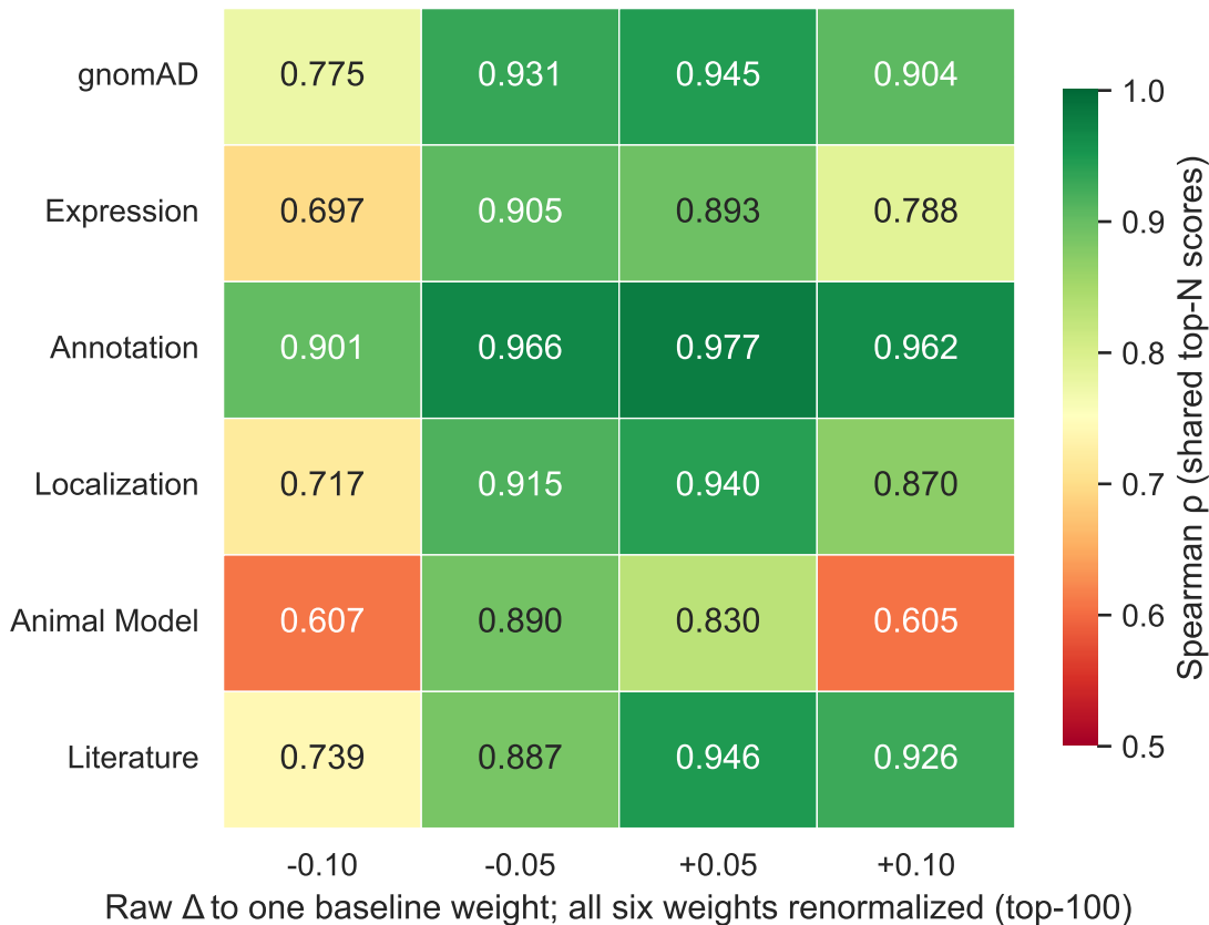
Weight perturbation sensitivity: Spearman \rho on shared top-100 genes
