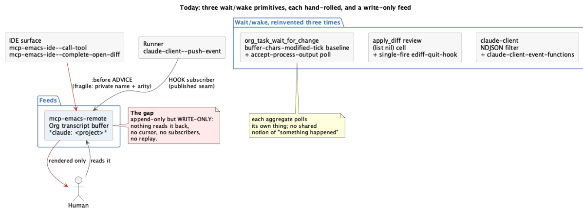
Figure 26.2: Today: three hand-rolled wait/wake primitives and a write-only feed
