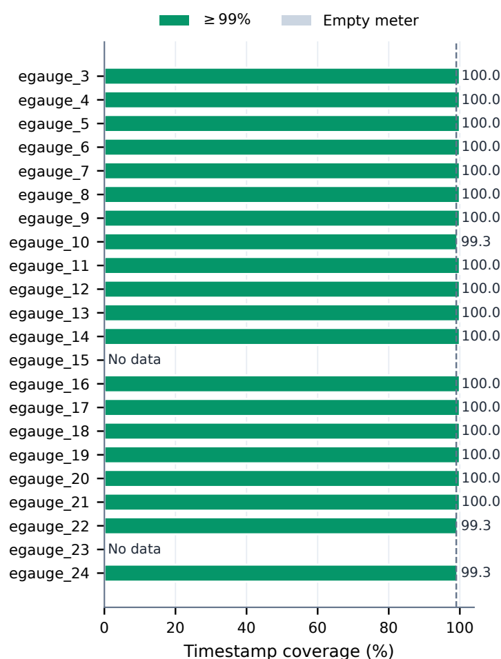
Figure 4.13. Meter-level voltage timestamp coverage during the available normal-operation baseline.
