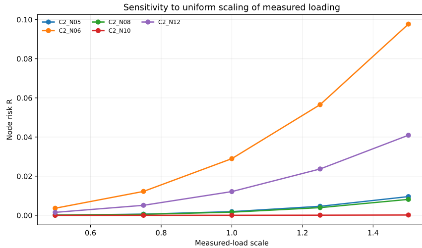
Figure 4.15. Component 2 response to uniform counterfactual scaling of measured edge loading with root disturbance fixed at 0.75.
