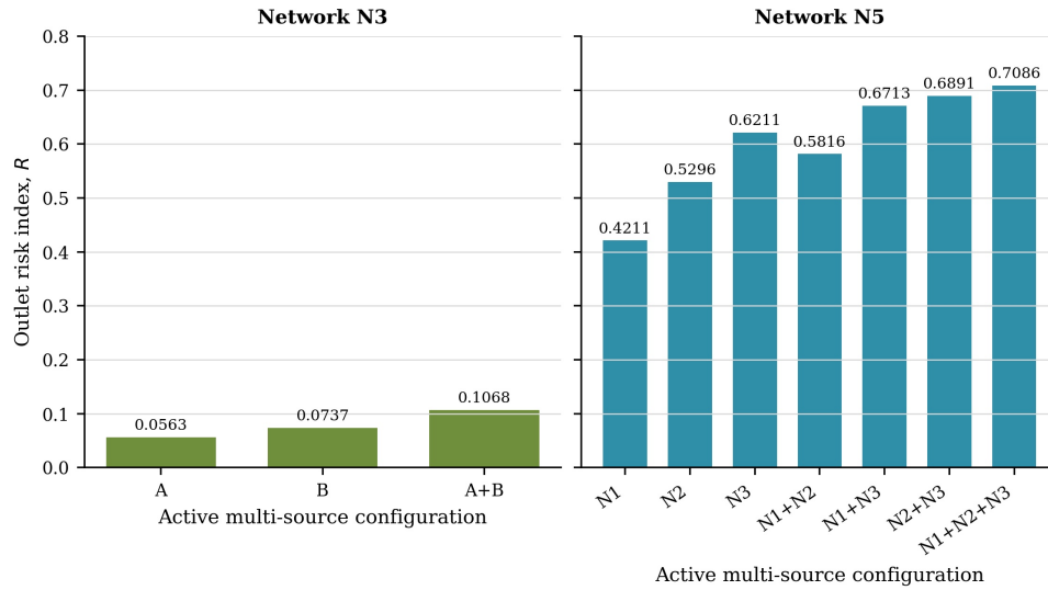
Figure 4.5. Outlet-risk response under single- and multi-source configurations in N3 and N5.
