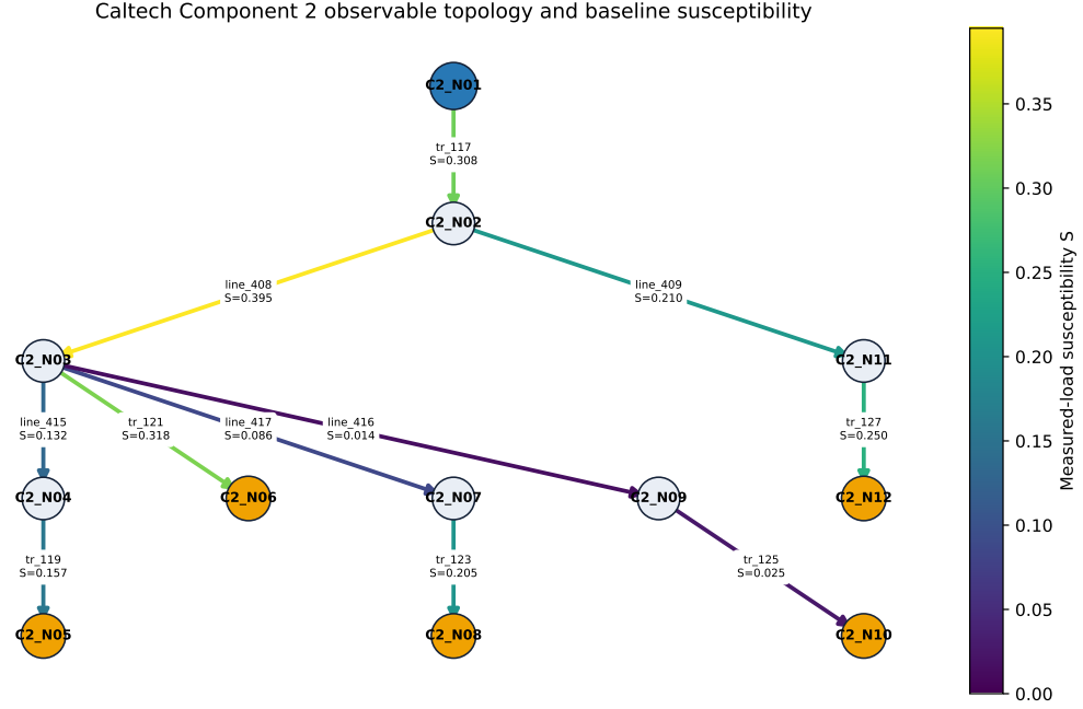
Figure 4.14. Observable Component 2 topology and baseline edge susceptibility derived from measured downstream apparent power and declared capacity.
