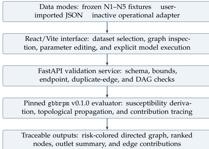
Figure 3.3. Research prototype architecture and separation between data modes, interface, validation service, versioned evaluator, and comparative outputs.
