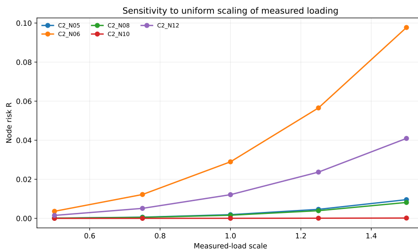
Figure 4.15. Component 2 response to uniform counterfactual scaling of measured edge loading with root disturbance fixed at 0.75.
