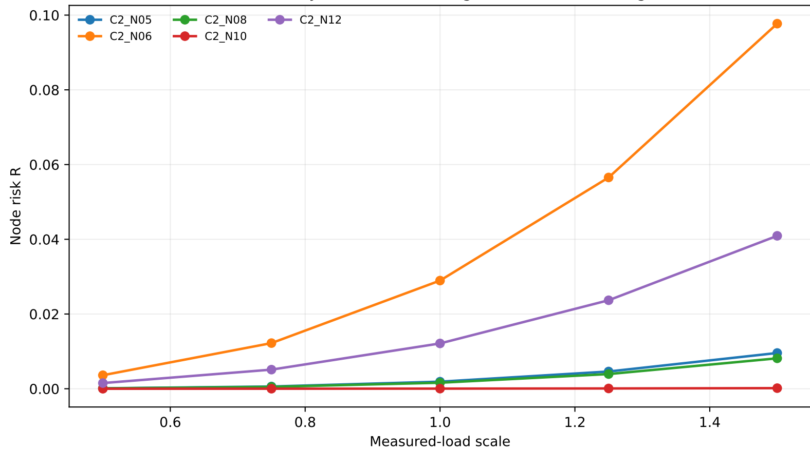
Sensitivity to uniform scaling of measured loading
