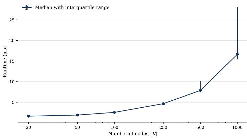
Figure 4.8. Median runtime and interquartile range of the one-pass GBBRPM evaluator on sparse DAGs.
