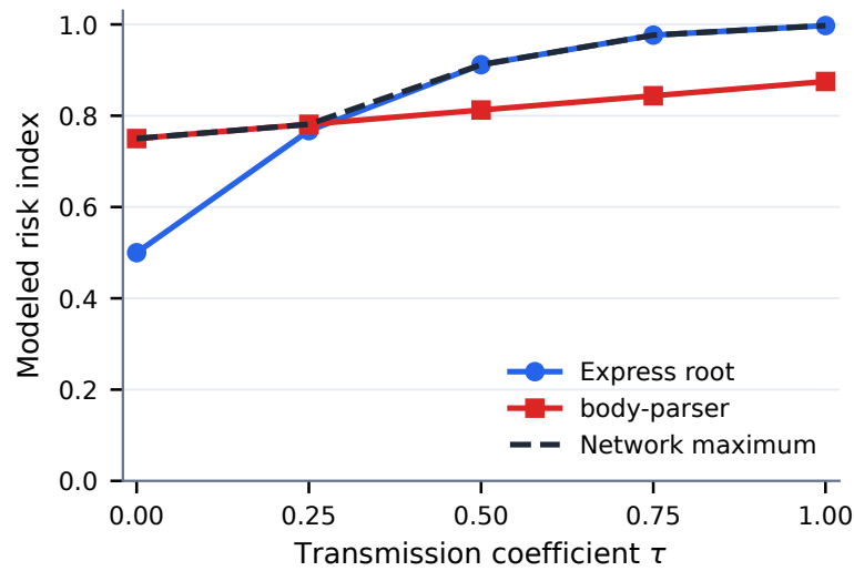
Figure 4.11. Modeled software risk across the transmission-coefficient sweep.
