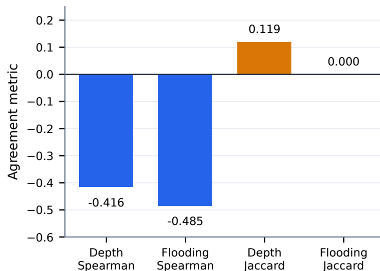
Figure 4.9. Agreement between GBBRPM priority changes and SWMM hydraulic outcomes across the 12 blockage scenarios.
