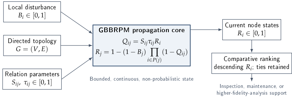
Figure 1.1. Conceptual framework of GBBRPM, distinguishing supplied domain inputs, the generic propagation core, and the comparative decision-support output.
