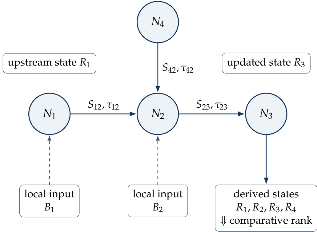
Figure 3.1. Generic directed-node example showing local inputs, relation-level modifiers, recursive state propagation, convergence at N_2 , and ranking from the computed node states.
