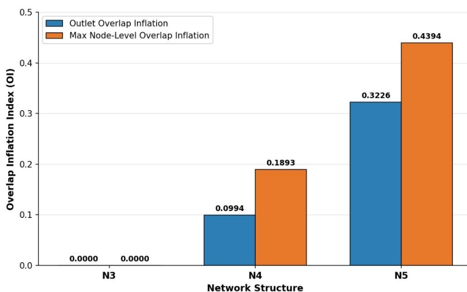
Figure 4.7. Overlap-inflation diagnostic for converging and reconverging networks.
