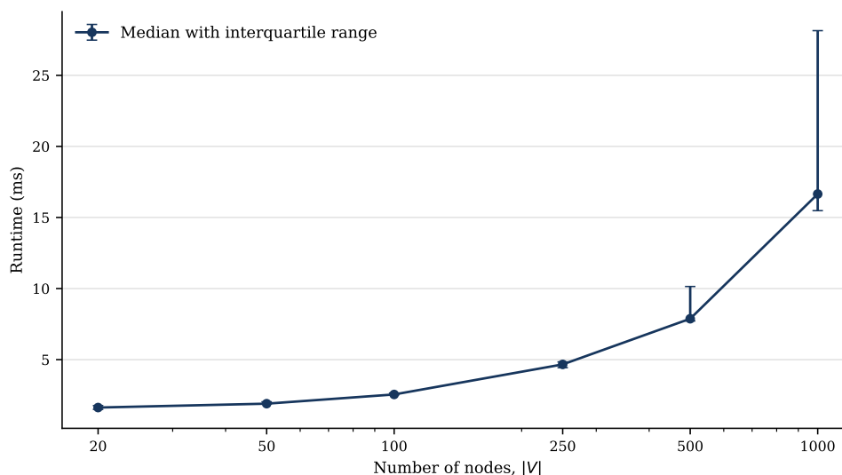
Figure 4.8. Median runtime and interquartile range of the one-pass GBBRPM evaluator on sparse DAGs.
