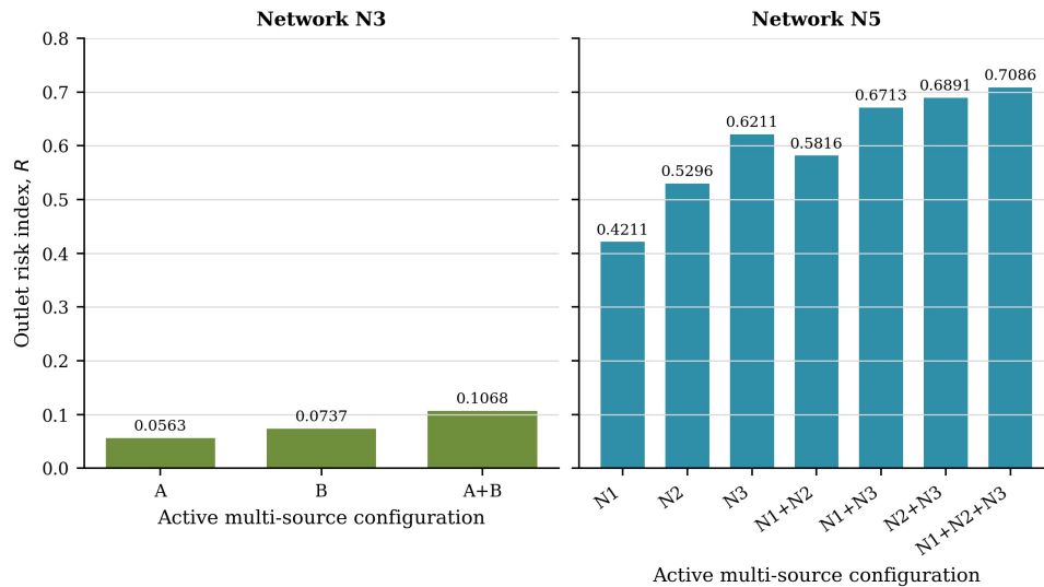
Figure 4.5. Outlet-risk response under single- and multi-source configurations in N3 and N5.
