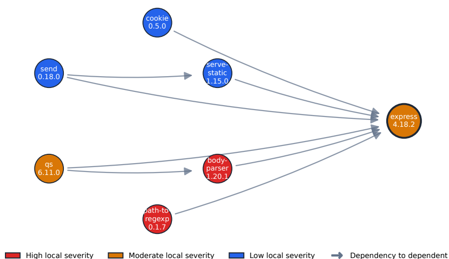
Figure 4.10. Evidence-backed vulnerable packages and their directed dependency relations to the Express root.
