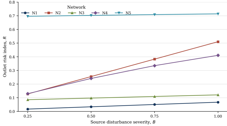
Figure 4.2. Outlet-risk response to increasing source disturbance severity across N1–N5.
