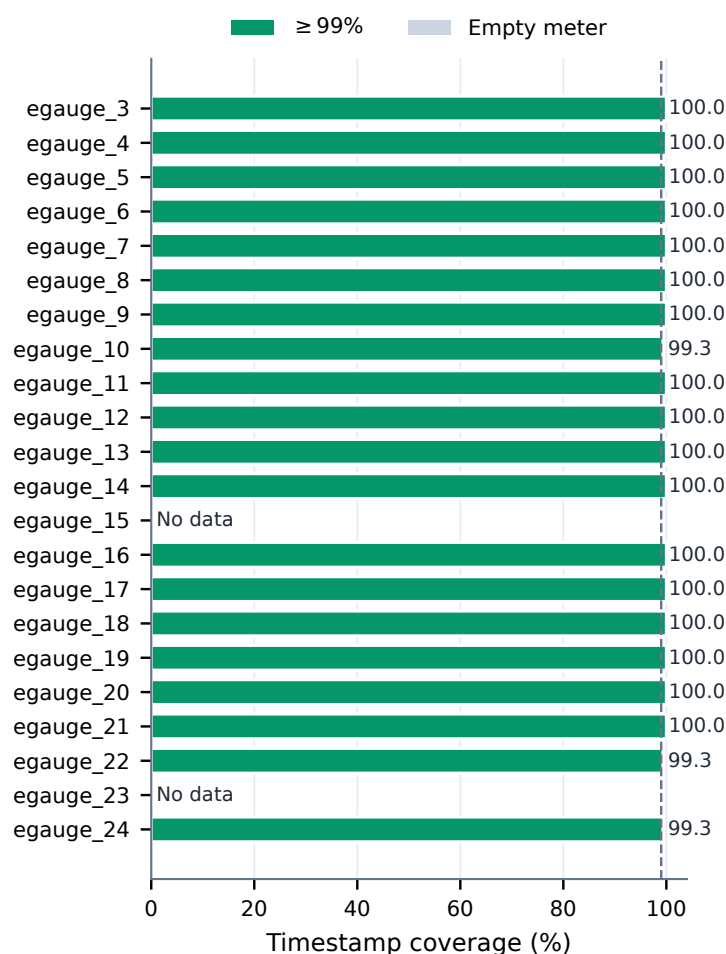
Figure 4.13. Meter-level voltage timestamp coverage during the available normal-operation baseline.
