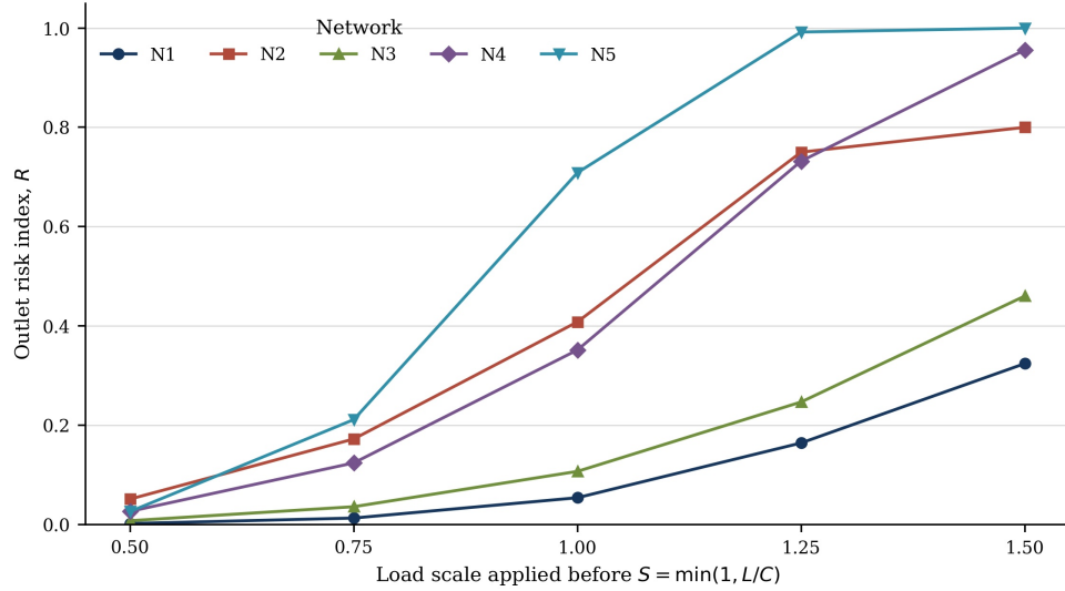
Figure 4.3. Outlet-risk response to increasing L/C stress under bounded susceptibility.
