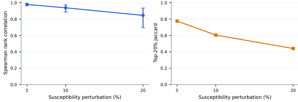
Figure 4.6. Drainage ranking stability under \pm 5\% , \pm 10\% , and \pm 20\% susceptibility perturbations. Error bars show the reproduced Spearman distribution; the second panel reports top-20% Jaccard overlap.
