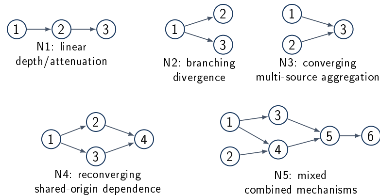
Figure 3.2. Controlled synthetic DAG set. Node labels identify evaluation order; arrows indicate permitted propagation direction.
