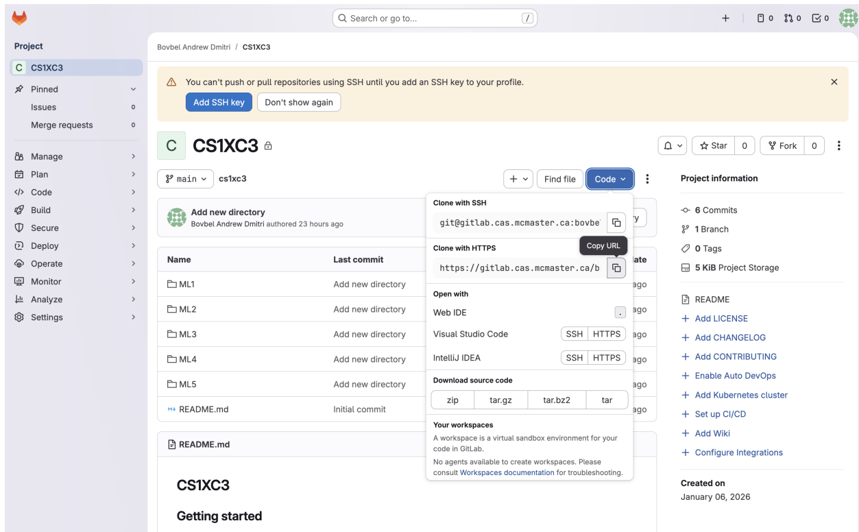
Figure 9: Where to find the code button
