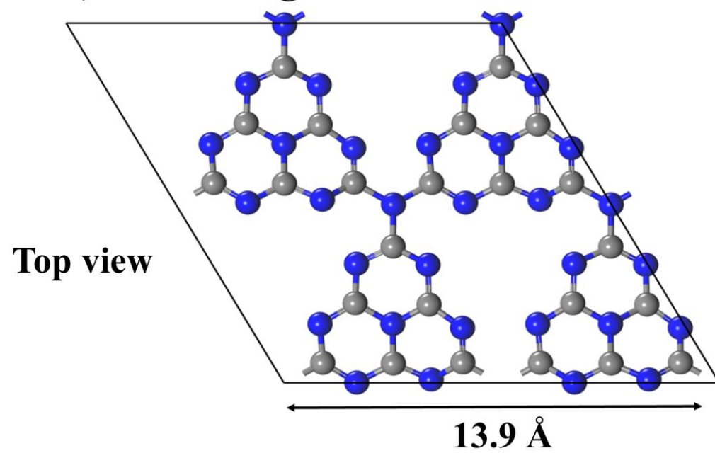
b) Buckled g-C 3 N 4
