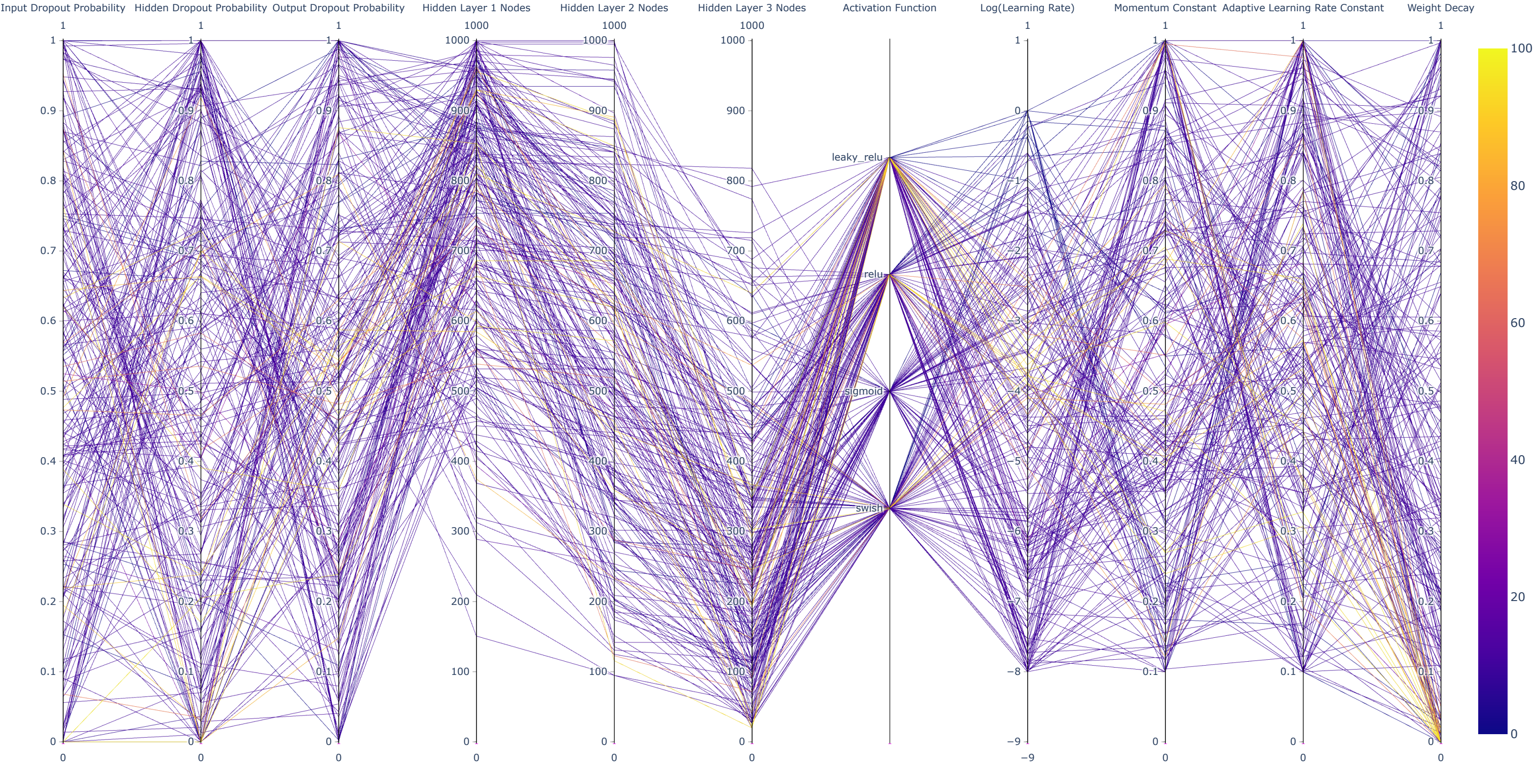
MNIST Test Accuracy Parallel Coordinate Plot, JES, Colored by Test Accuracy
