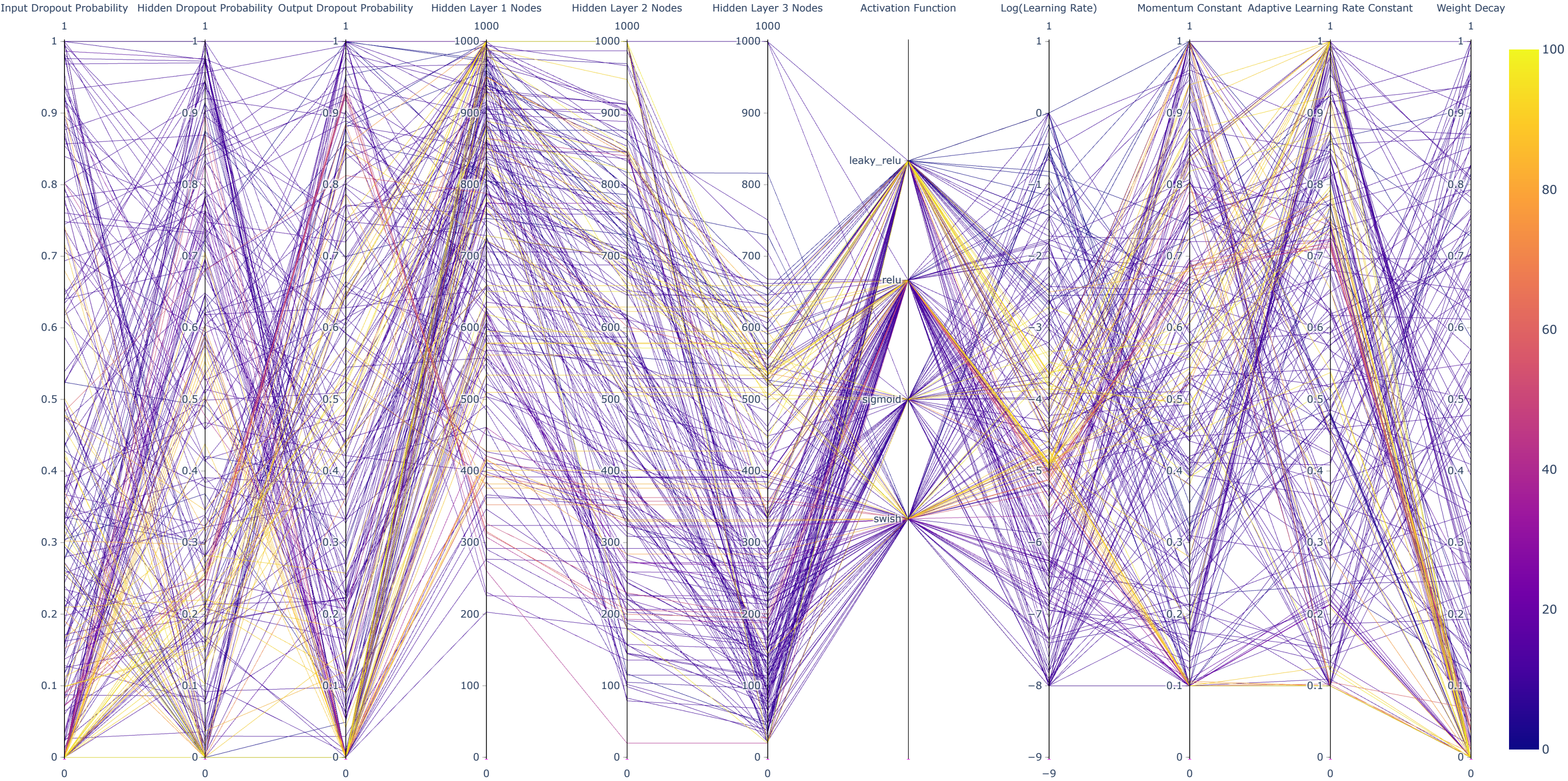
MNIST Test Accuracy Parallel Coordinate Plot, LogNEI, Colored by Test Accuracy
