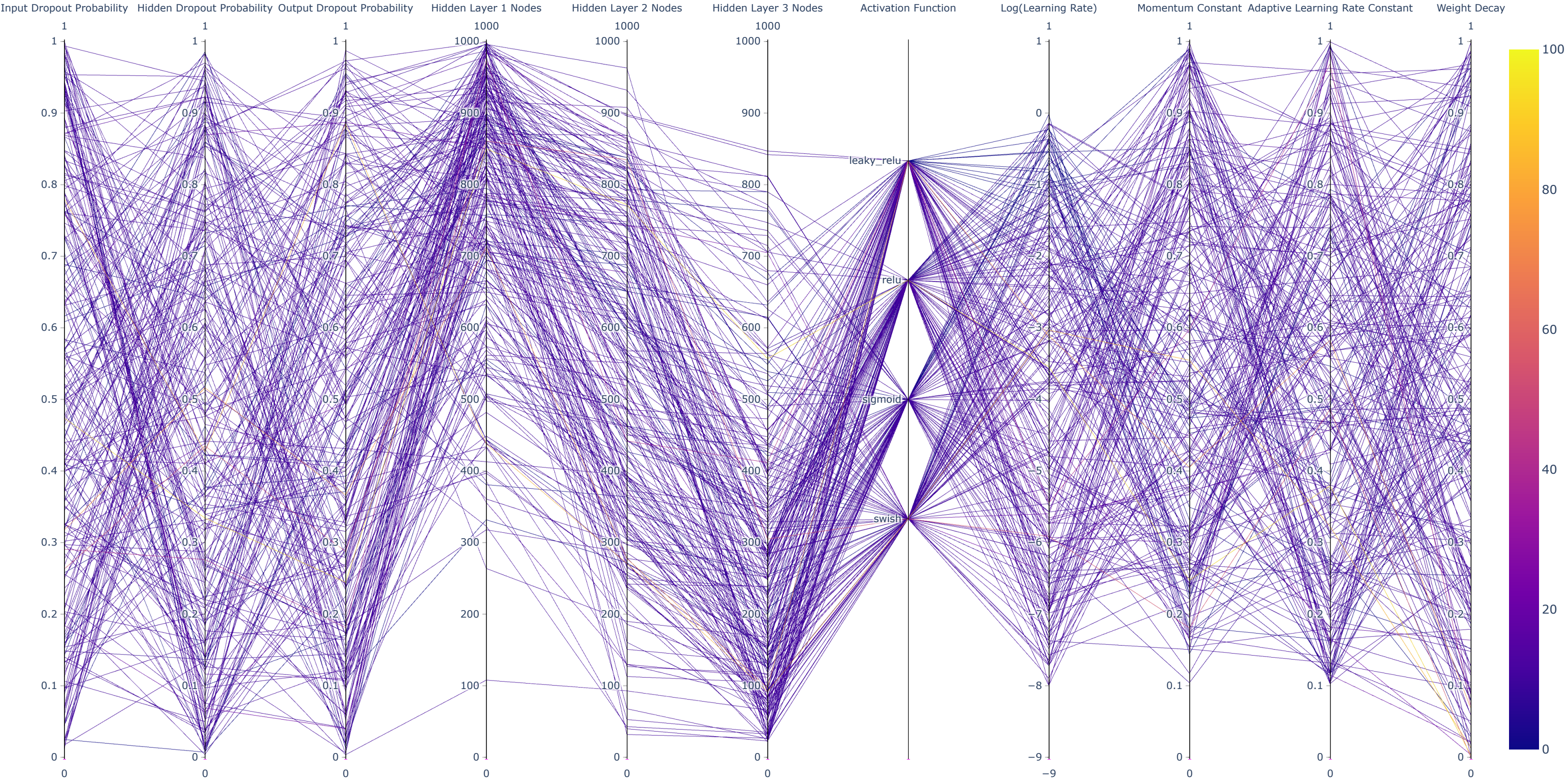
MNIST Test Accuracy Parallel Coordinate Plot, Random Search, Colored by Test Accuracy
