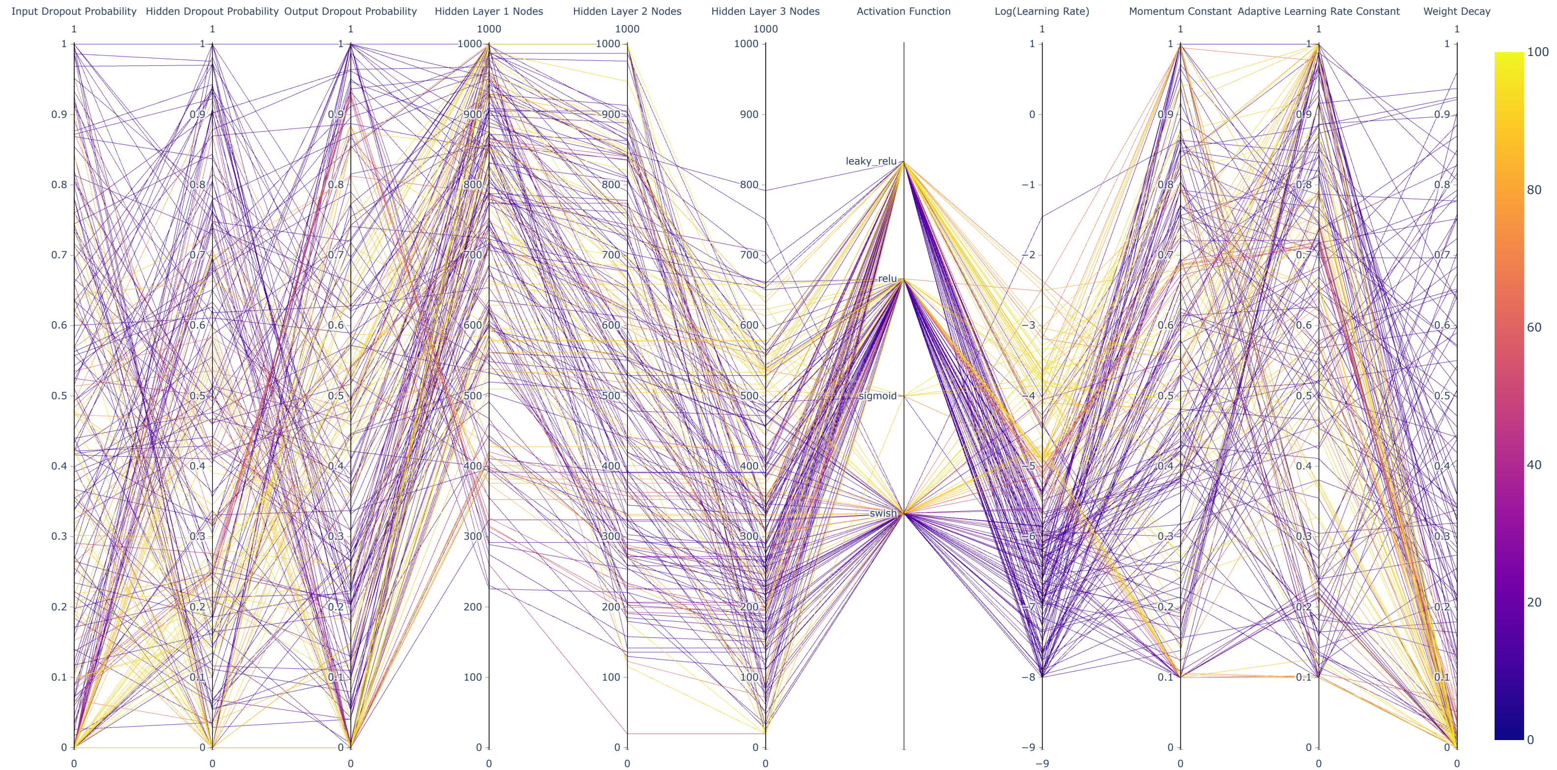
MNIST Test Accuracy Parallel Coordinate Plot, Hyperparameters Above Median, Colored by Test Accuracy
