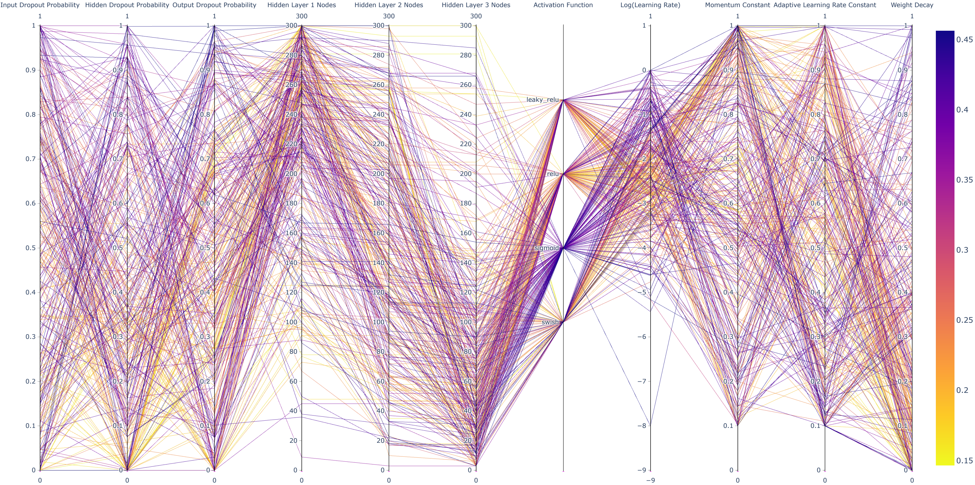
Superconductivity Test Normalized RMSE Parallel Coordinate Plot, Hyperparameters Above Median, Colored by NRMSE
