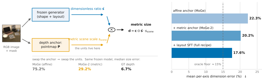
Fig. 1: Metric scale is delegated to the depth anchor. Left: a depth-conditioned image-to-3D generator predicts only a dimensionless object–scene ratio \hat{s} ; physical units enter exclusively through the scene scale s_{\text{scene}} of the conditioning pointmap (Eq. 2). Swapping the anchor on the same frozen model moves median size error from 75.2% (affine MoGe) to 6.7% (ground-truth depth) with zero trained parameters (Table 1). Right: exploiting delegation — a metric monocular anchor plus light layout fine-tuning approaches the oracle isotropic-correction floor (Table 2), using no ground-truth depth.
