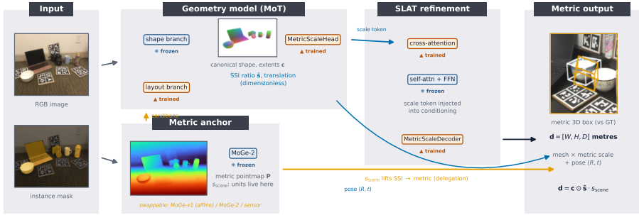
Fig. 2: Pipeline. A single RGB image and instance mask condition two paths: the frozen MoGe-2 anchor supplies the metric pointmap \mathbf{P} and scene scale s_{\text{scene}} (swappable — the delegation slot), while the Mixture-of-Transformers geometry model predicts canonical shape (frozen branch) and dimensionless layout (trained branch). The trained MetricScaleHead summarises shape and anchor statistics into a scale token injected into the SLAT refiner’s cross-attention (the only trained SLAT weights); the MetricScaleDecoder reads the refined latent into metric [W, H, D] . All metric outputs inherit their units from the anchor via \mathbf{d} = \mathbf{c} \odot \tilde{\mathbf{s}} \cdot s_{\text{scene}} .
