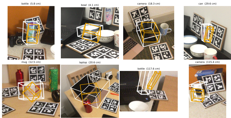
Fig. 2: Predicted metric 3D boxes (orange) vs. ground truth (white) on NOCS-Real275, RGB-only inference with the MoGe-2 anchor. Panel titles give the class and translation error. The first six panels span the six categories; the last two show the characteristic failure mode — distant, partially occluded cameras and bottles where the monocular anchor’s depth error displaces the box along the viewing ray.
