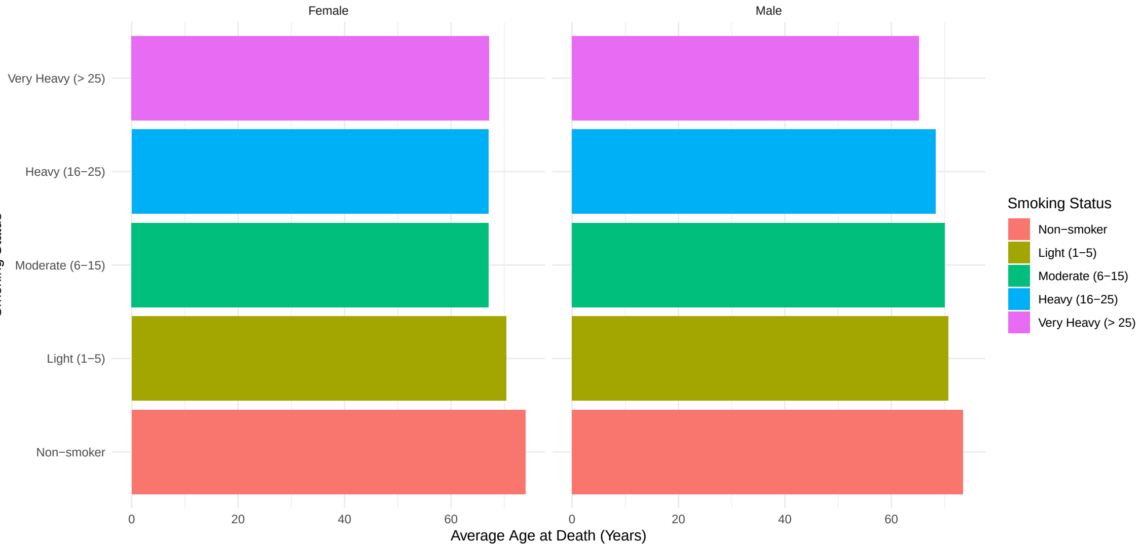
Average Age at Death by Smoking Status and Sex
