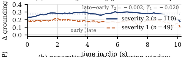
(a) FineLAP grounding gain vs. time in clip
