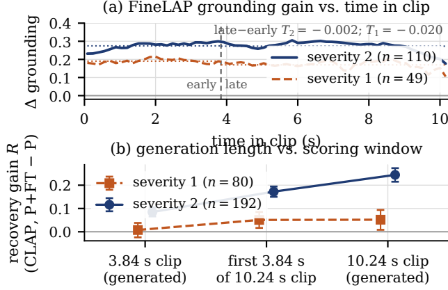
Fig. 2. (a) FineLAP frame-level grounding gain (P+FT - P) vs. time in the 10.24s clip (vertical line: 3.84s): uniform, not back-loaded. (b) R (95% CI) on the generated 3.84s clip, the first 3.84s of the 10.24s clip and the full clip: a generation-length, not scoring-window, effect.
