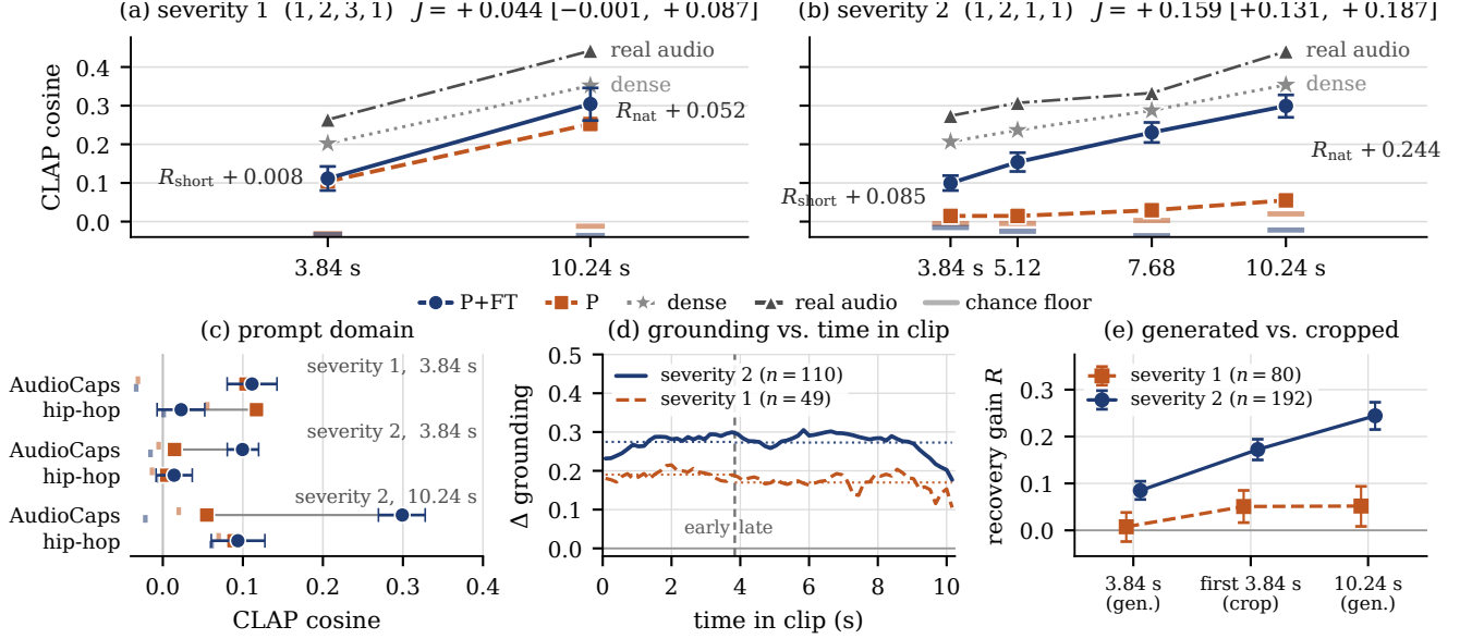
Fig. 1. The recovery gain across the operating points we measure ( n as in Sec. 3.2). Duration , mean CLAP cosine of the pruned (P) and fine-tuned (P+FT) checkpoints against generated clip duration at (a) severity 1 and (b) severity 2, with the real audio of the same prompts, each cell’s chance floor and the matched dense control (same prompts and scoring convention); whiskers are the 95% CI of the paired gain R about the P+FT mean, and J = R_{\text{nat}} - R_{\text{short}} . Domain , (c) the same two checkpoints on in-domain AudioCaps and on held-out hip-hop captions per (severity, duration) cell, each against its own chance floor. Where the gain sits , (d) FineLAP frame-level grounding gain (P+FT – P) vs. time in the 10.24 s clip—uniform, not back-loaded—and (e) R on the generated 3.84 s clip, on the first 3.84 s of the 10.24 s clip and on the full clip: a generation-length, not a scoring-window, effect.
