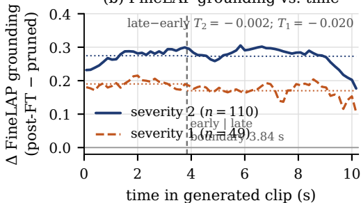
(b) FineLAP grounding vs. time
