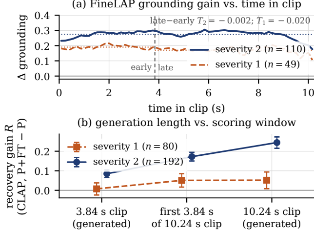
Fig. 2. (a) FineLAP frame-level grounding gain (P+FT - P) vs. time in the 10.24s clip (vertical line: 3.84s): uniform, not back-loaded. (b) R (95% CI) on the generated 3.84s clip, the first 3.84s of the 10.24s clip and the full clip: a generation-length, not scoring-window, effect.
