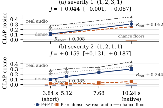
Fig. 1. The recovery gain grows with clip duration. Mean CLAP cosine of the pruned (P, dashed) and fine-tuned (P+FT, solid) checkpoints at the short and native points, (a) severity 1, and (b) severity 2 with the two sweep durations; whiskers: 95% CI of the paired gain R about the P+FT mean. Anchors: real audio of the same prompts (triangles), each cell’s chance floor (ticks) and the matched dense control (stars; same prompts and scoring convention).
