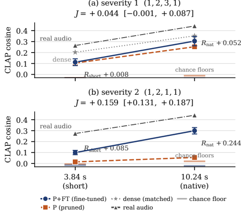
Fig. 1. The recovery gain grows with clip duration. Mean CLAP cosine of the pruned (P, dashed) and fine-tuned (P+FT, solid) checkpoints at the short and native points for (a) severity 1 and (b) severity 2; whiskers: 95% CI of the paired gain R , drawn about the P+FT mean; J annotated. Anchors: the real audio of the same prompts (triangles, dash-dot) and each cell’s shuffled-caption chance floor (short ticks). Panel (a) includes the matched dense control (stars; same 80 prompts, same scoring convention).
