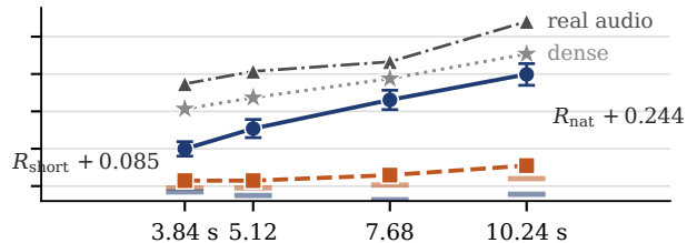
(b) severity 2 (1, 2, 1, 1) J = +0.159 [+0.131, +0.187]
