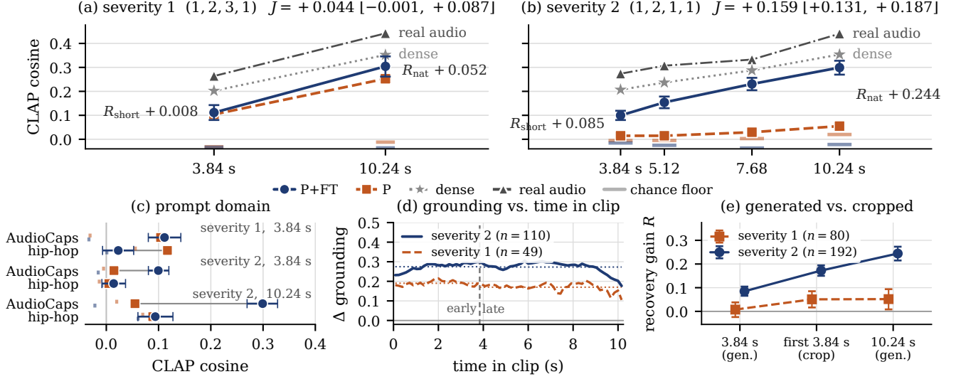
Fig. 1. The recovery gain across the operating points we measure ( n as in Sec. 3.2; whiskers are 95% CIs of R ). Duration: mean CLAP cosine of P and P+FT against generated clip duration at (a) severity 1 and (b) severity 2, with the real audio of the same prompts, each cell’s chance floor and the matched dense control; J = R_{\text{nat}} - R_{\text{short}} . Domain: (c) the same checkpoints in-domain and on held-out hip-hop captions, per (severity, duration) cell, against their own floors. Where: (d) FineLAP grounding gain vs. time in the 10.24s clip; (e) R on the generated 3.84s clip, on its first 3.84s and on the full clip.
