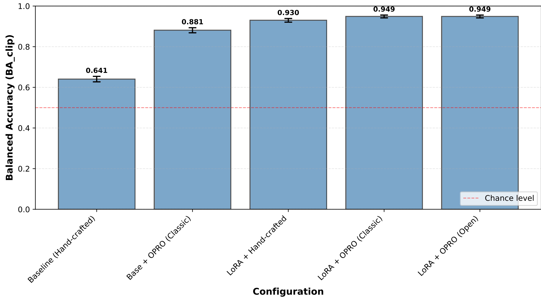
Overall Performance: Balanced Accuracy Across Configurations
