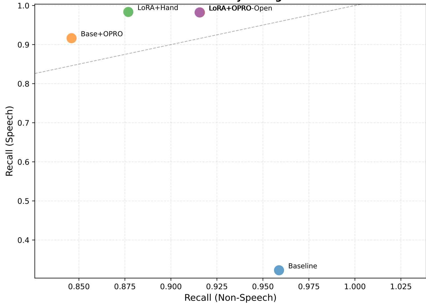
Recall Trade-off by Configuration
