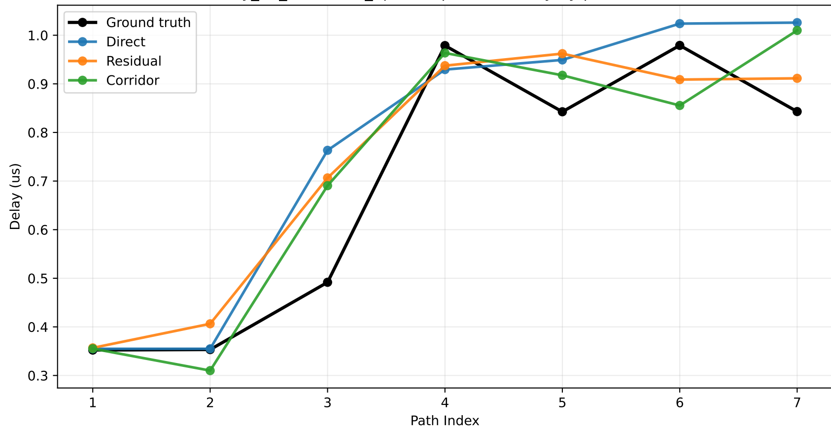
city_31_barcelona_3p5 sample 192: delay by path index
