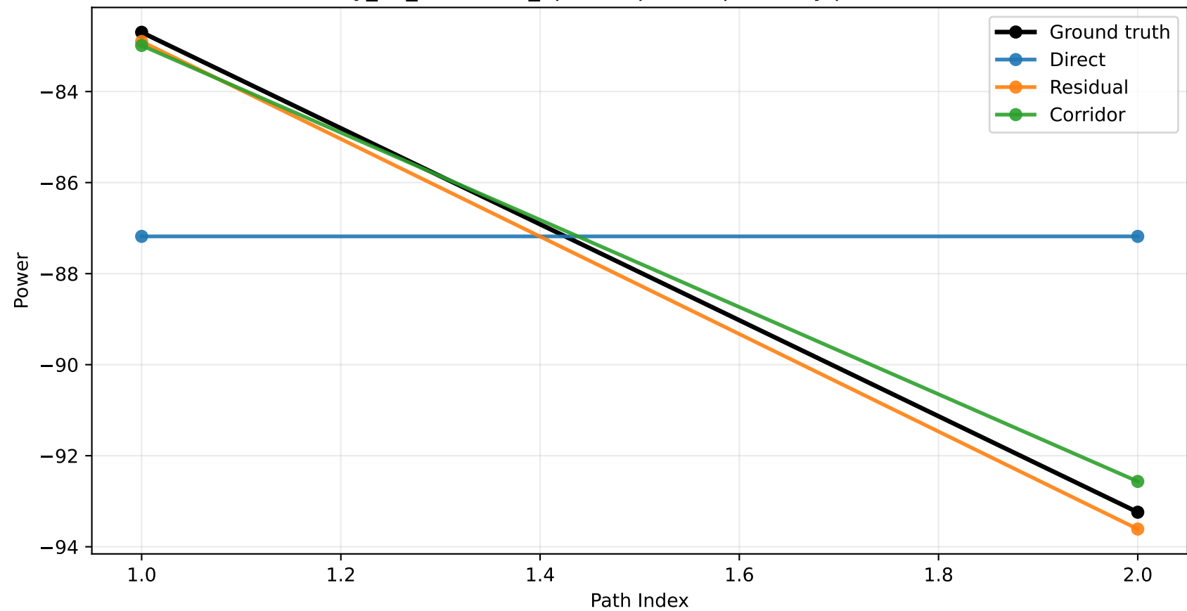
city_31_barcelona_3p5 sample 25: power by path index
