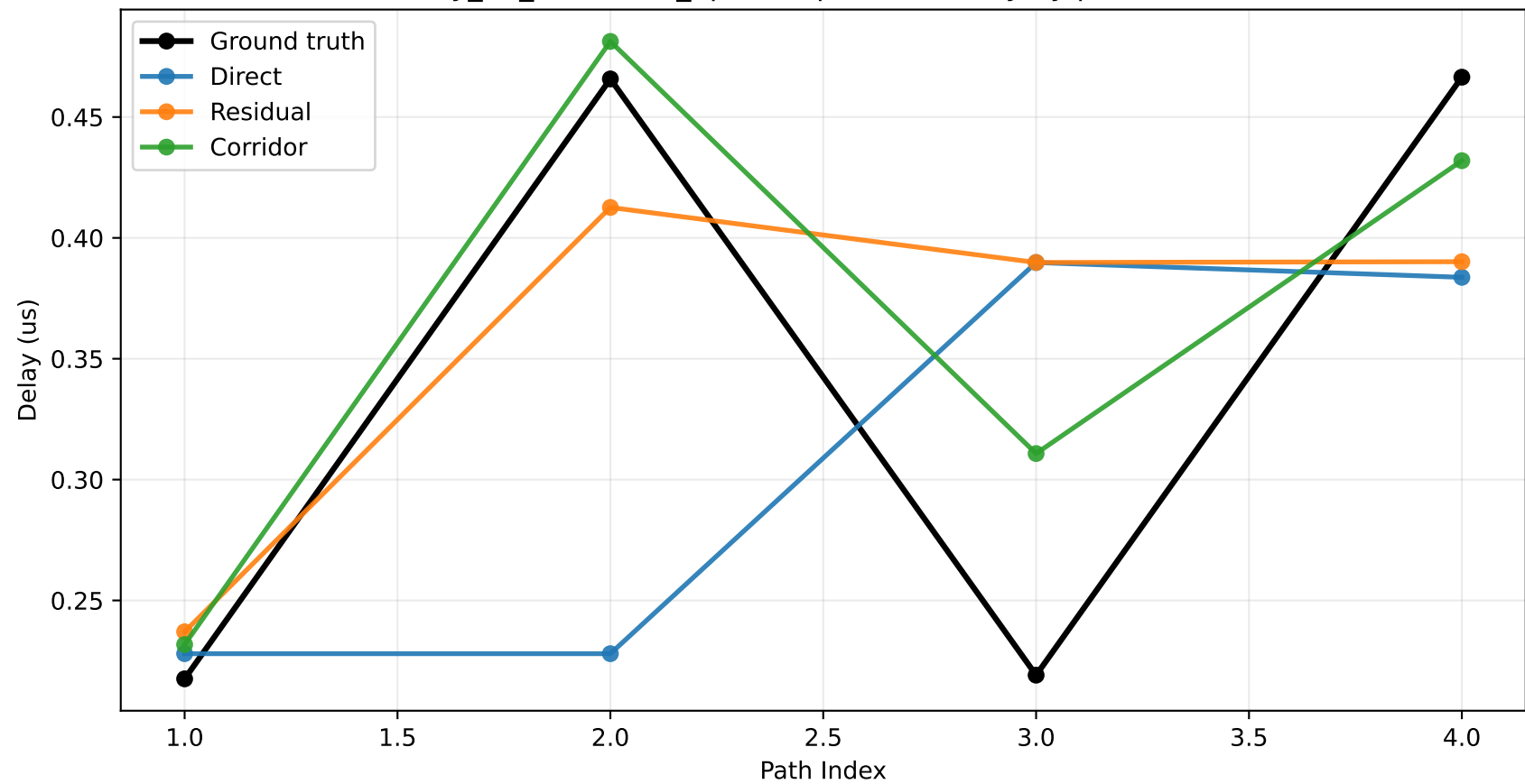
city_31_barcelona_3p5 sample 430: delay by path index
