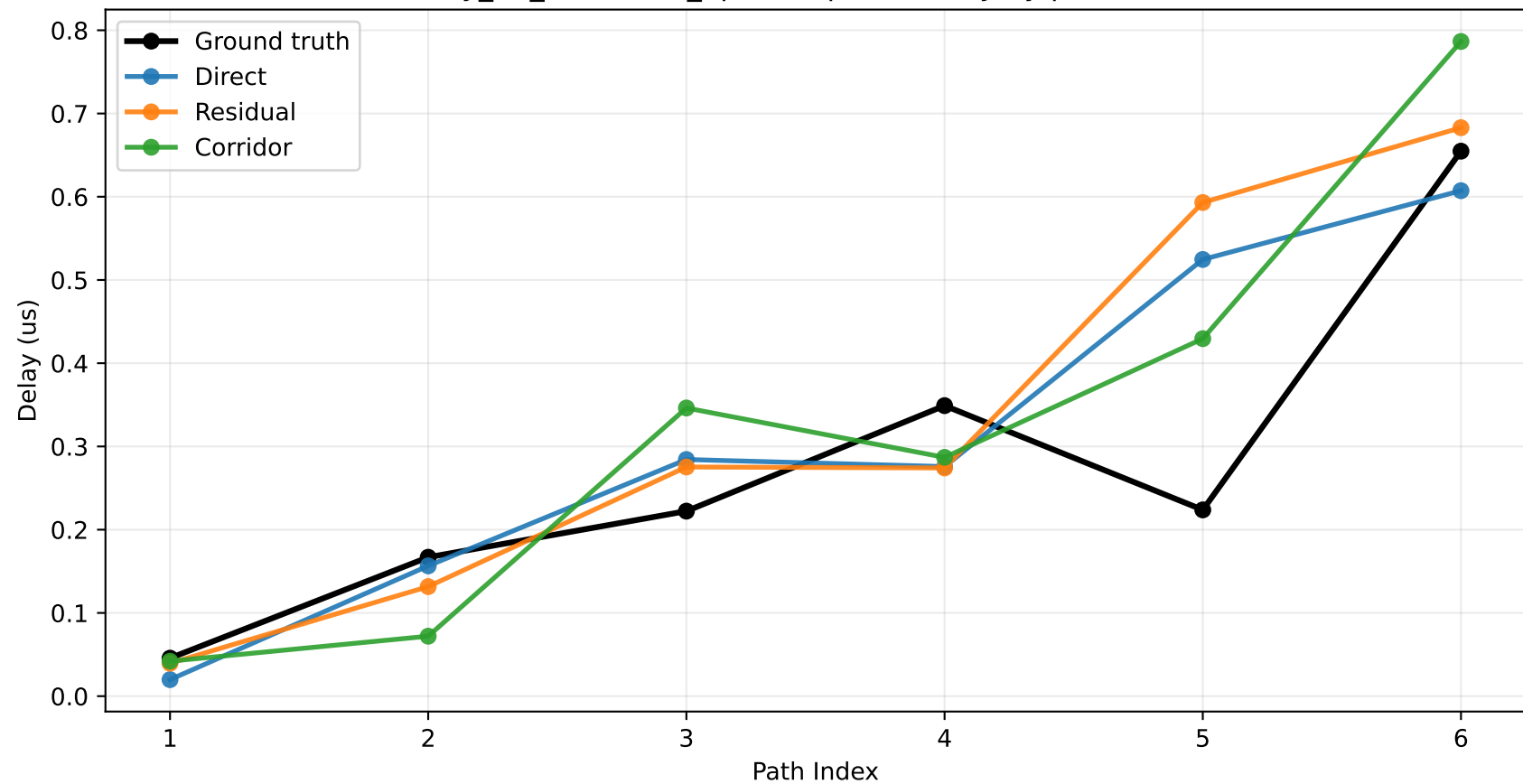
city_31_barcelona_3p5 sample 5: delay by path index
