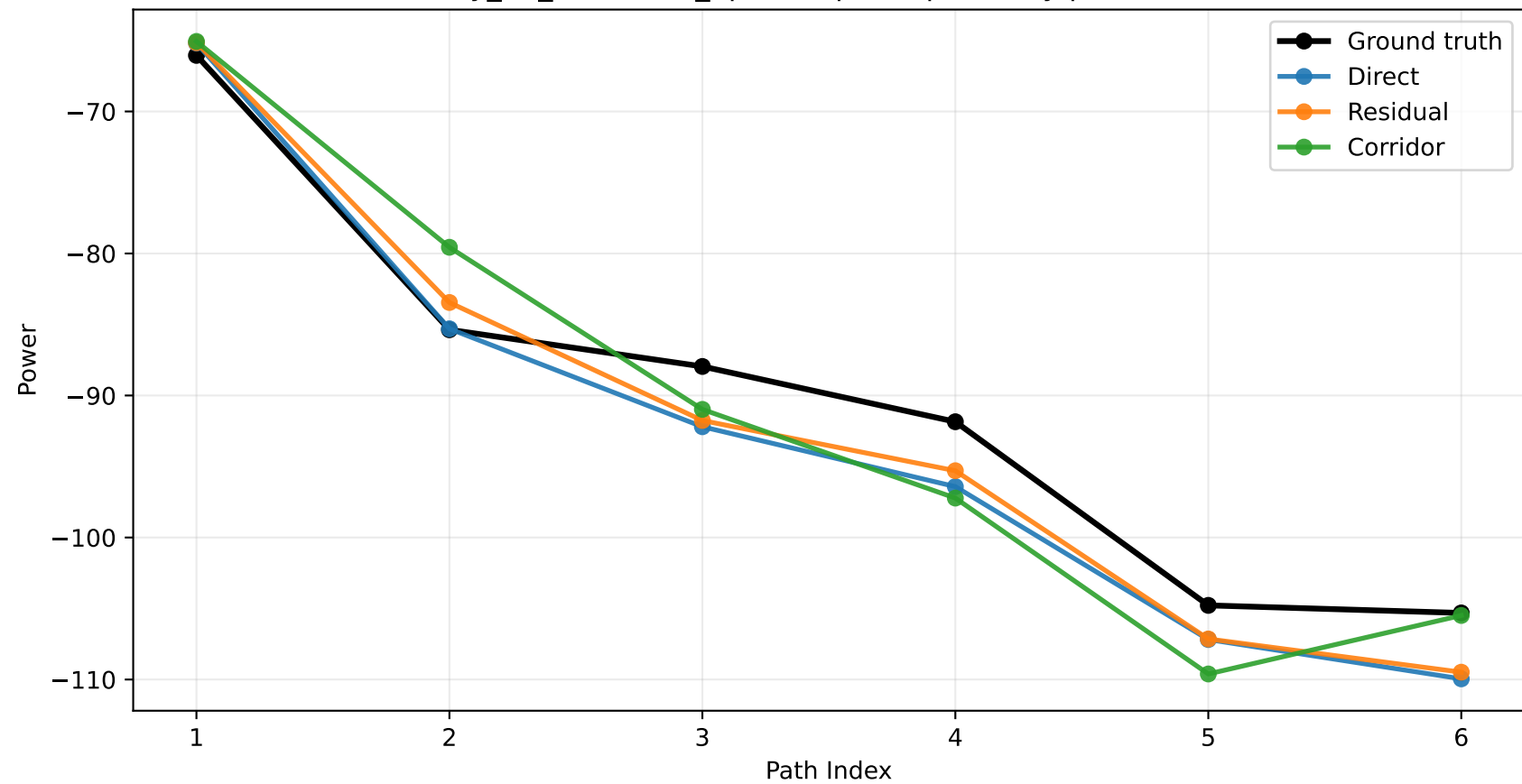
city_31_barcelona_3p5 sample 5: power by path index
