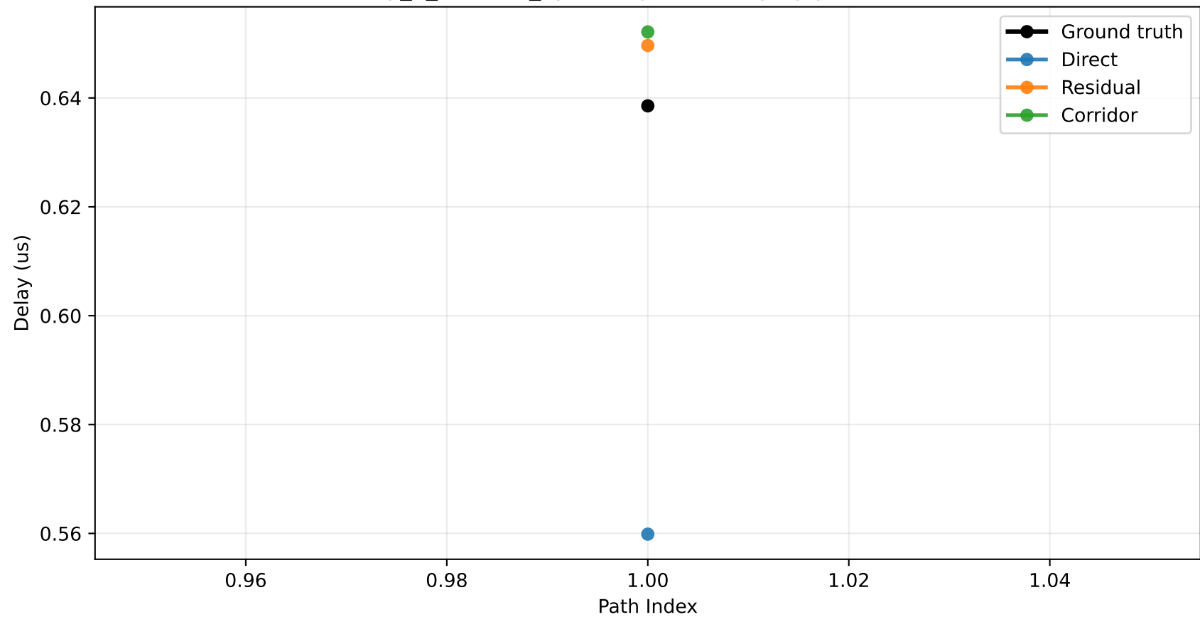
city_3_houston_3p5 sample 0: delay by path index
