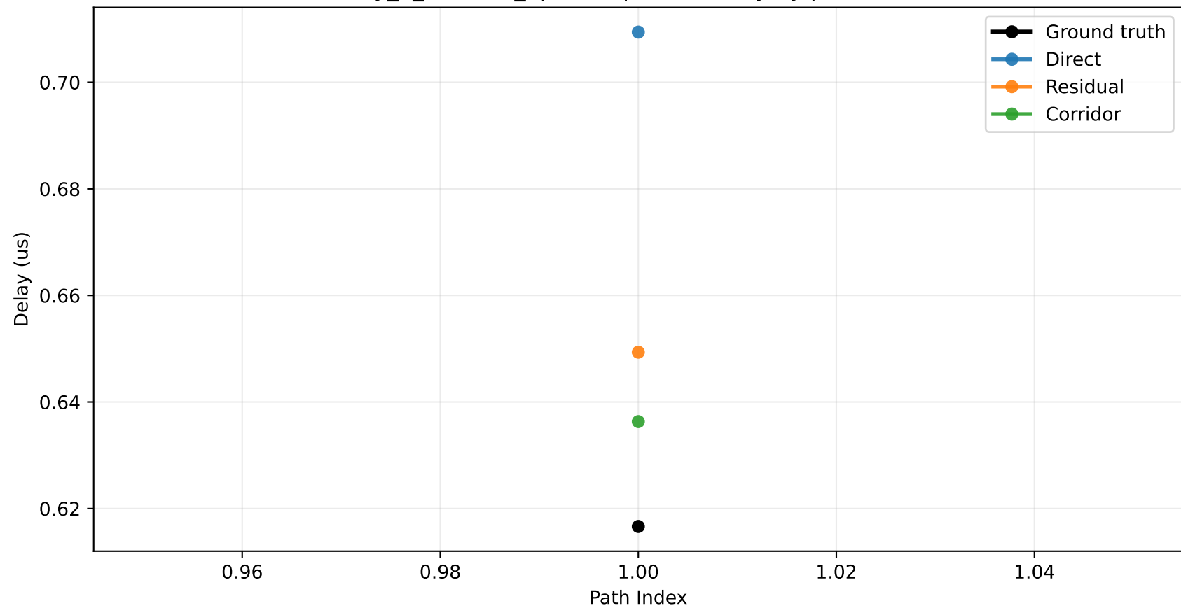
city_3_houston_3p5 sample 92: delay by path index
