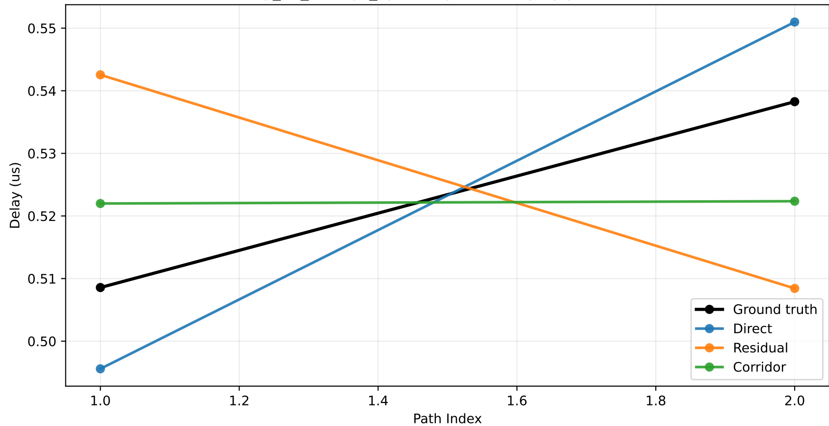
city_47_chicago_3p5 sample 0: delay by path index
