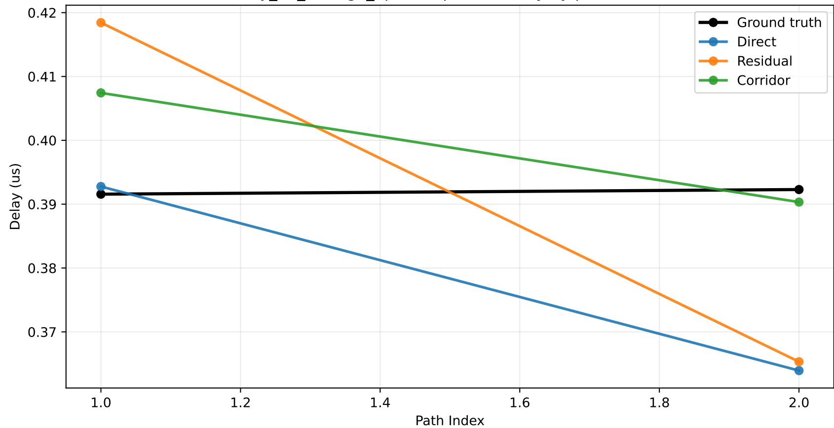
city_47_chicago_3p5 sample 10: delay by path index
